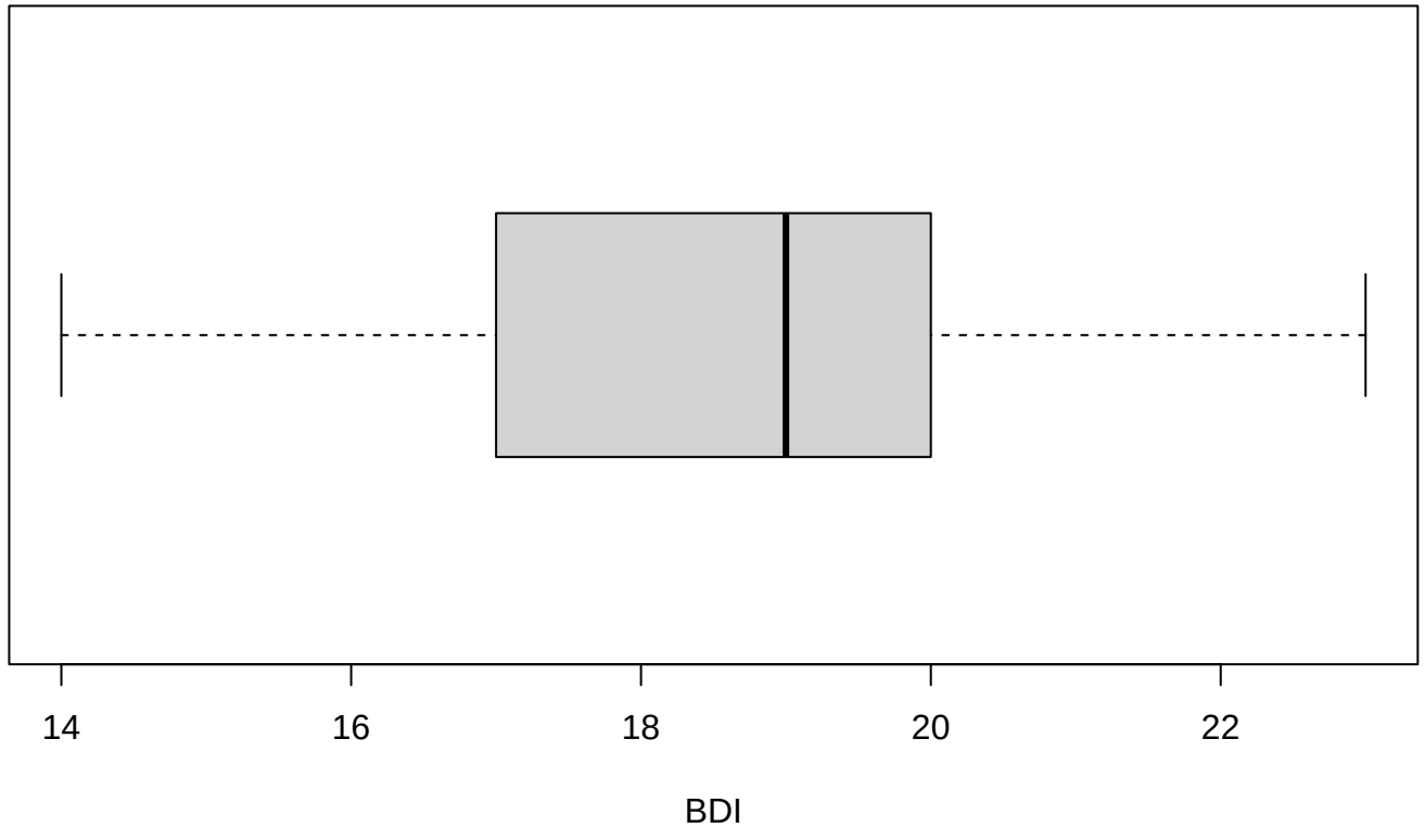
Boxplot
