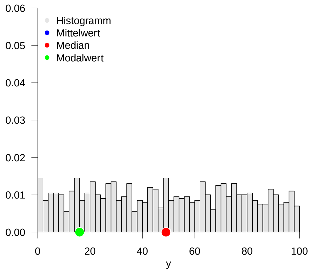
C Mittelwert = 49.1, Median = 49.0, Modalwert = 16.0
