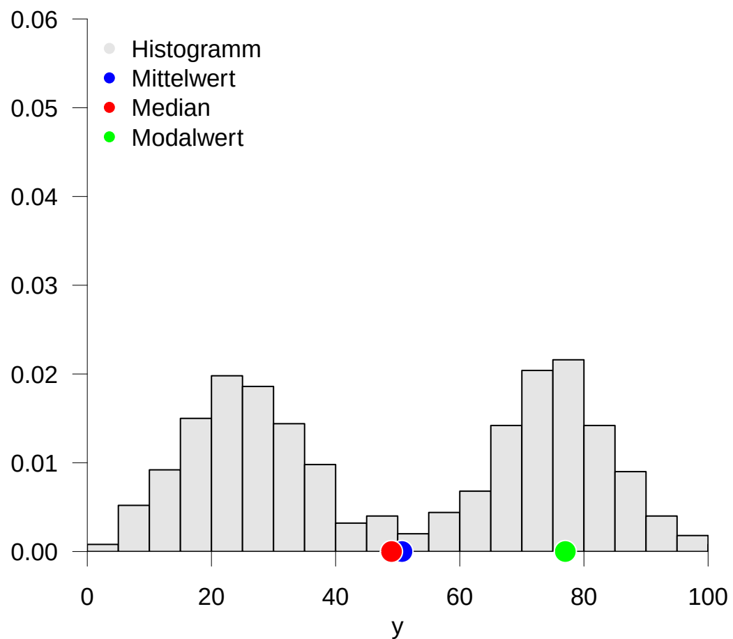
B Mittelwert = 50.7, Median = 49.0, Modalwert = 77.0
