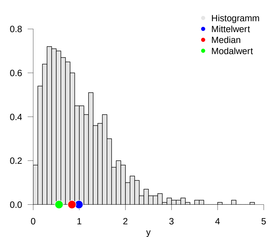
D Mittelwert = 1.0, Median = 0.8, Modalwert = 0.6
