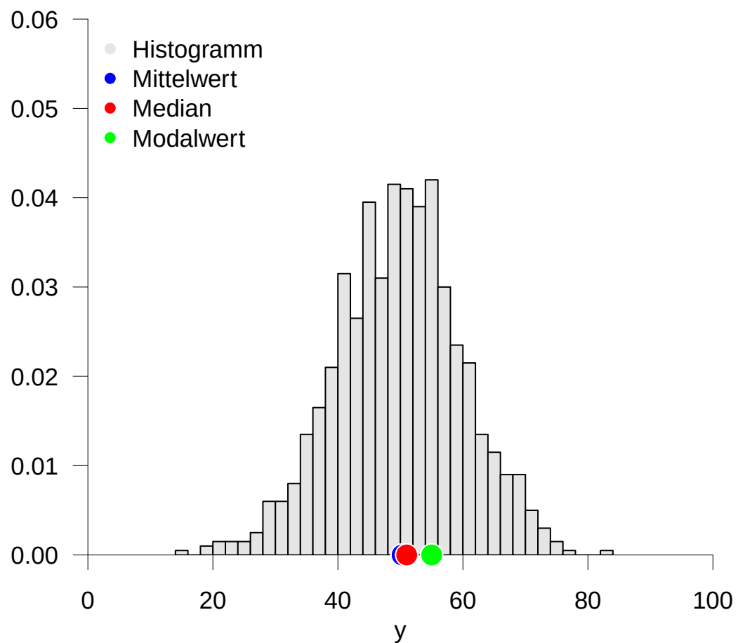
A Mittelwert = 50.3, Median = 51.0, Modalwert = 55.0
