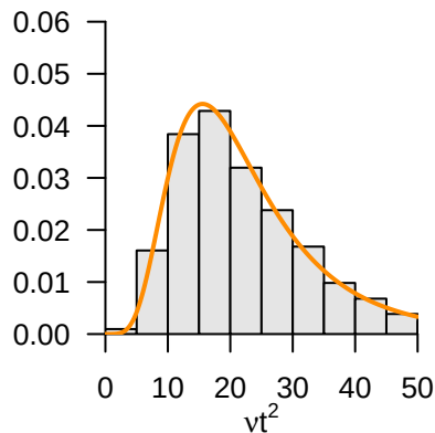
B \nu T^2 \sim f(\delta, m, n - m)
