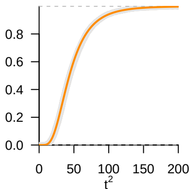
D P(t^2) := F(\nu t^2; \delta, m, n - m)
