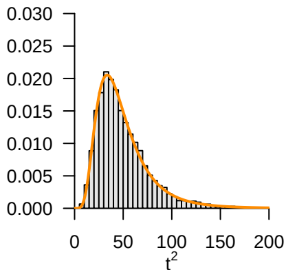
C p(t^2) := \nu f(\nu t^2; \delta, m, n - m)
