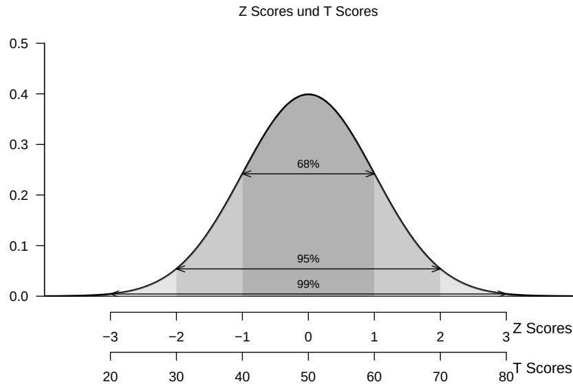
Figure 49.1 Z scores and T scores.
