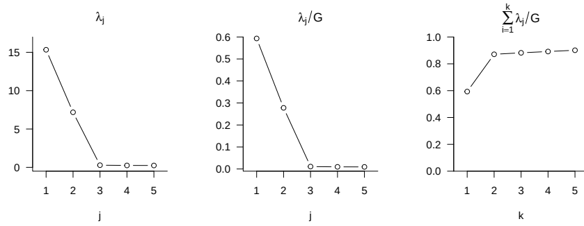
Figure 51.5 Scree plot and relative and cumulative total sample variance for increasing numbers of factors for the BDI-II data set according to Keller et al. (2008).
