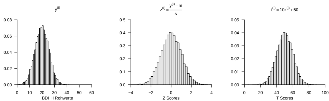
Figure 49.2 Simulated sample BDI-II raw scores, Z scores, and T scores
