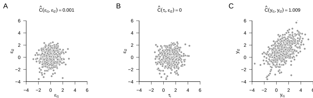
Figure 50.3 Normal distribution example regarding two parallel test measurements.
