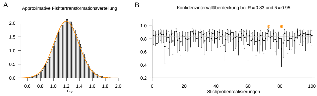
Figure 50.4 A Simulation of the distribution of the Fisher-transformed sample correlation and its analytical approximation. B Simulation of the coverage probability of the confidence interval for the sample correlation given a true, but unknown, correlation of R = 0.833 and a desired coverage probability of \delta := 0.95 . The figure shows the confidence interval and the corresponding sample correlation for each sample realization. In the present simulation, the confidence intervals cover the same true, but unknown, correlation R := 0.833 , shown by a gray line, in 98 out of 100 cases. The sample realizations for which this is not the case are marked with an orange circle.
