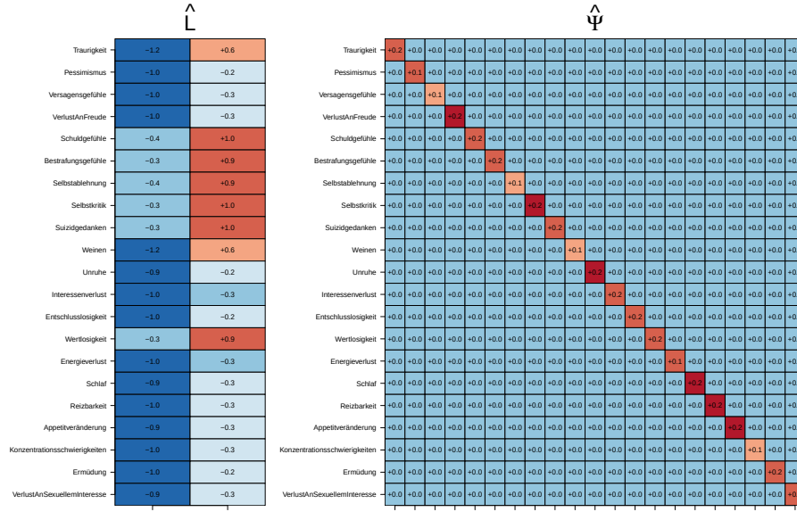
Figure 51.3 Factor loading matrix and specificity estimator for the BDI-II data set according to Keller et al. (2008).
