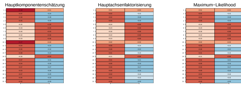
Figure 51.4 Factor loading matrix estimator for the BDI-II data set according to Keller et al. (2008) based on principal components, iterated principal axis factorization and maximum likelihood estimation
