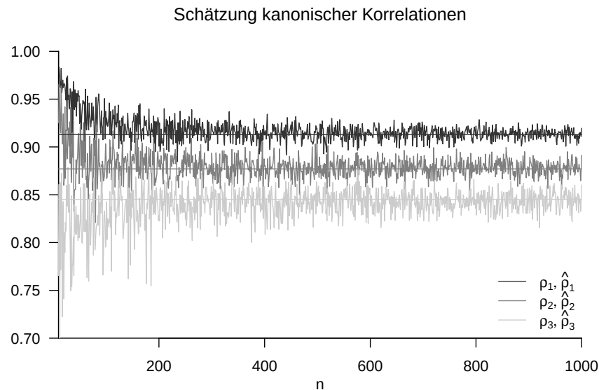
Figure 48.1 Estimation of canonical correlations in the simulation example
