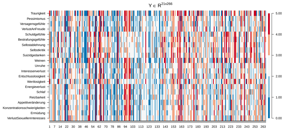
Figure 51.1 Simulated BDI-II data set according to Keller et al. (2008).
