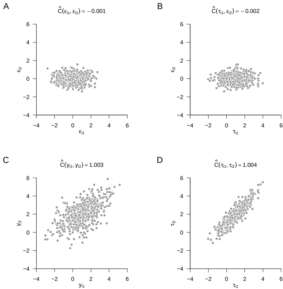
Figure 50.2 Normal distribution example for two test measurements.
