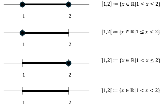
Figure 2.6 Representation of intervals on the number line. The black dot indicates that the corresponding number is part of the interval.
