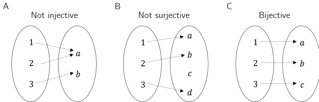
Figure 4.3 Injectivity, surjectivity, bijectivity.
