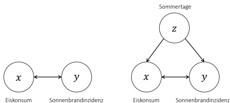
Figure 43.2 Random variables in the example scenario.
