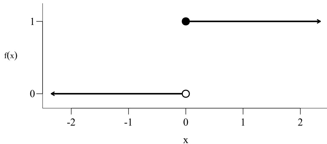
Figure 5.5 Heaviside function with f(0) = 1 .
