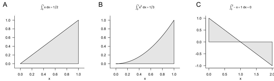
Figure 7.7 Examples of the second fundamental theorem of calculus
