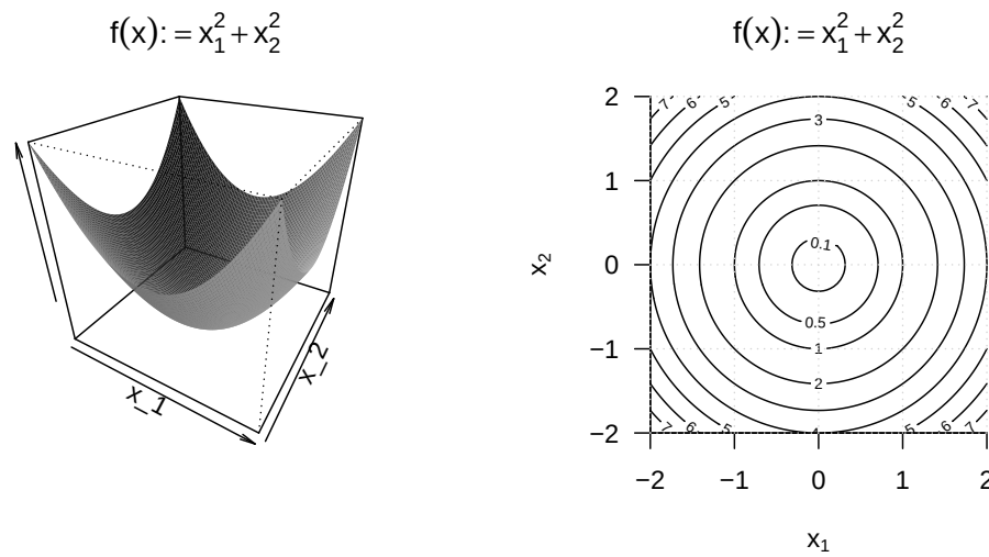
Figure 6.6 Visualizations of a bivariate function. The left-hand panel visualizes the function values as a surface above the two-dimensional domain of the function. Although this representation has a certain three-dimensional character, it is a bivariate function with a correspondingly two-dimensional domain. The right-hand panel visualizes lines with equal function values in the two-dimensional domain of the function.
