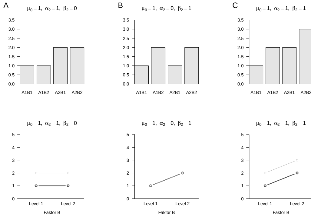
Figure 42.4 Group expectation values of example parameter scenarios in bar- and line-plot form in the additive two-way ANOVA model.
