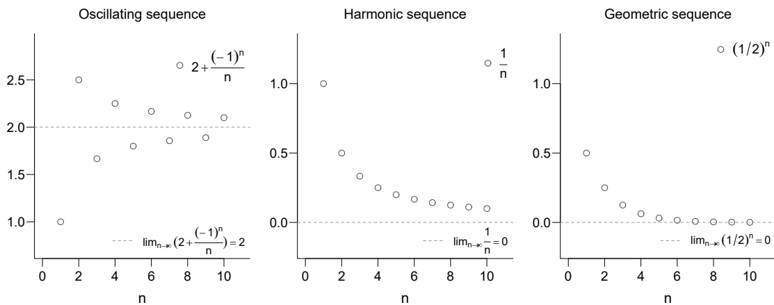
Figure 5.2 Limits of the oscillating, harmonic, and geometric sequences.
