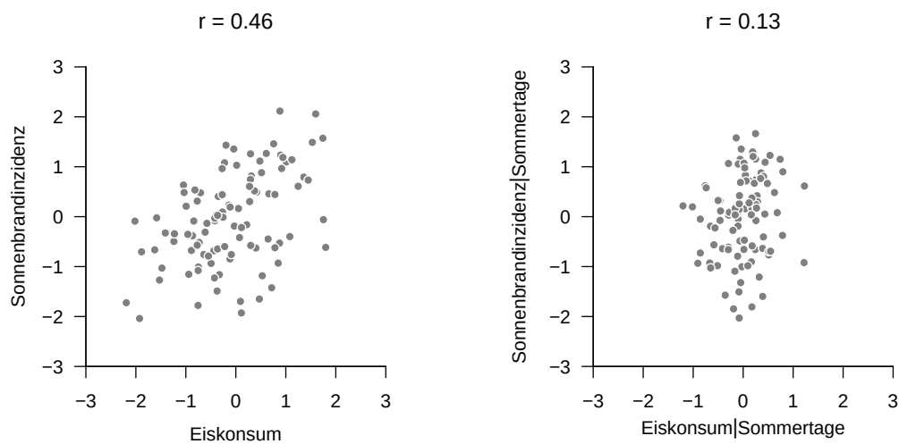
Figure 43.3 Evaluation of the partial correlation in the example scenario.
