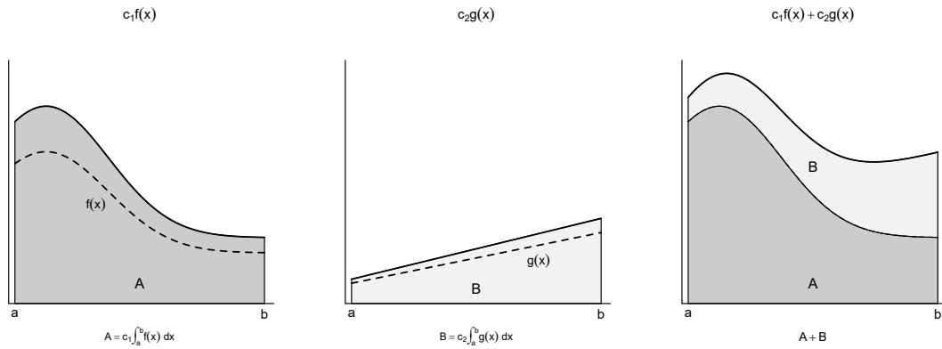
Figure 7.3 Linearity of definite integrals
