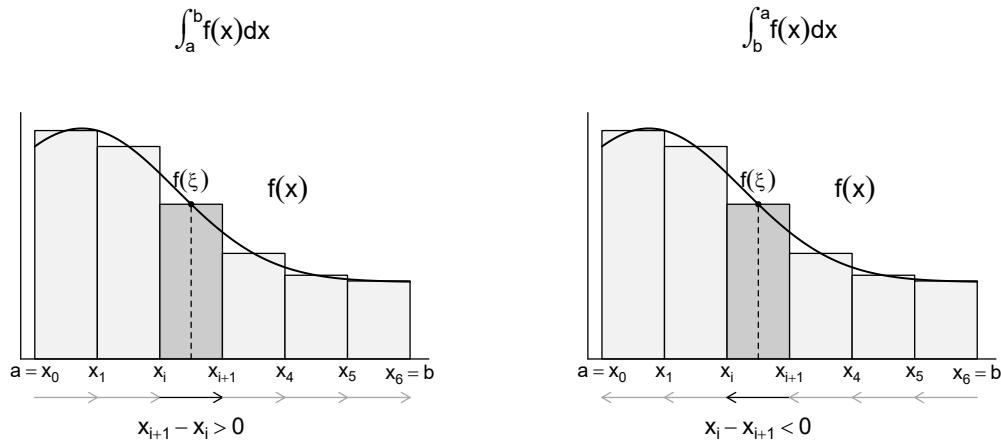
Figure 7.5 Orientation of definite integrals
