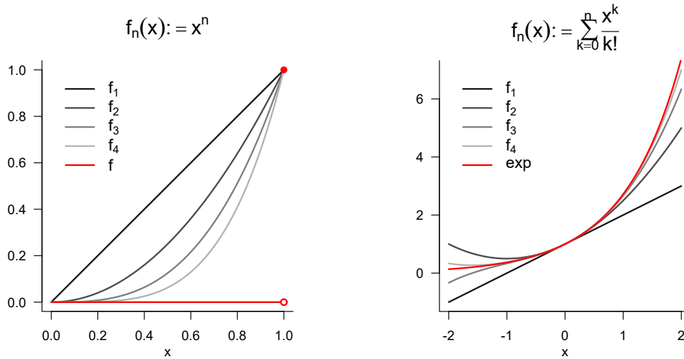
Figure 5.3 Examples of limits of sequences of functions.
