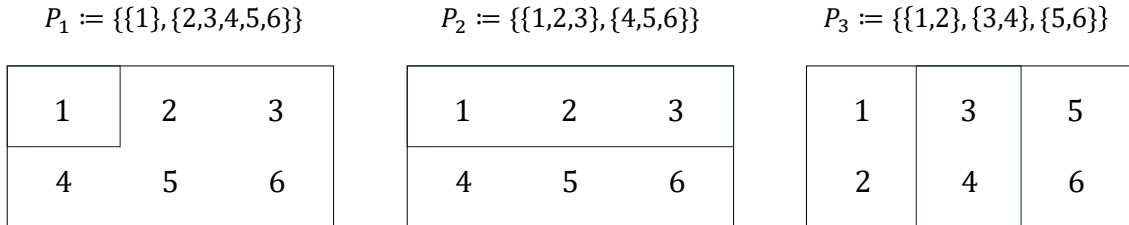
Figure 2.4 Diagrams of the partitions considered in the example for M := \{1, 2, 3, 4, 5, 6\} .
