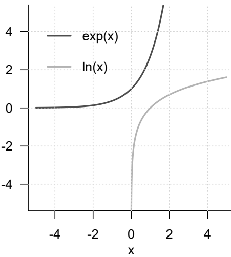
Figure 4.7 Exponential function and logarithm function
