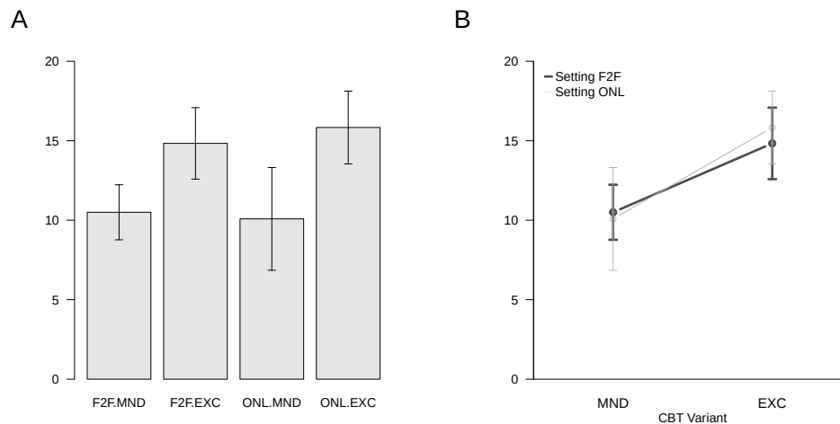
Figure 42.3 Visualization of the example data set as bar and line plots.
