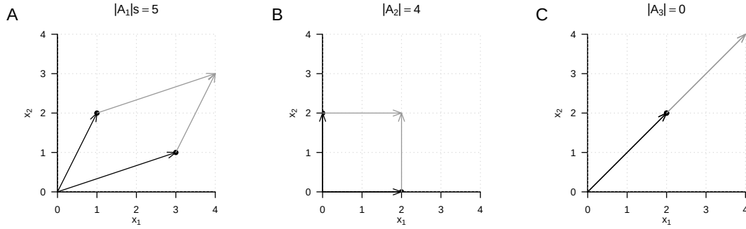
Figure 9.1 Determinants as parallelootope volumes.
