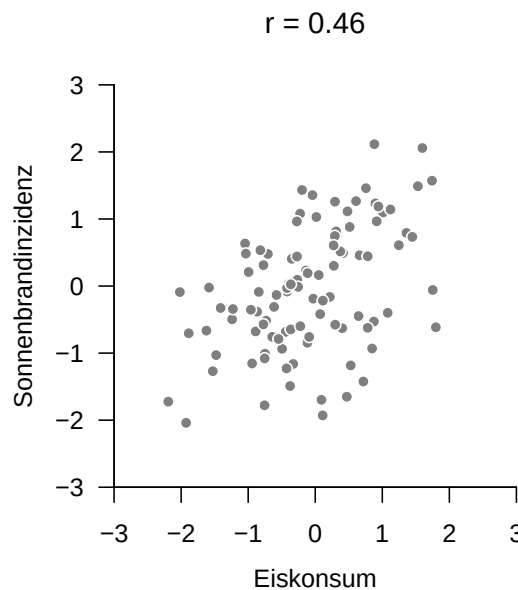
Figure 43.1 Example scenario for evaluating conditional and partial correlations.
