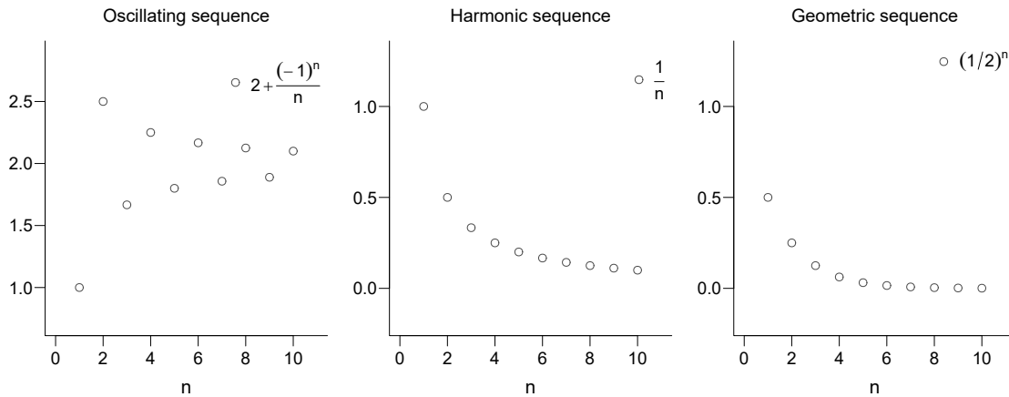
Figure 5.1 An oscillating sequence, a harmonic sequence, and a geometric sequence without their limits indicated.
