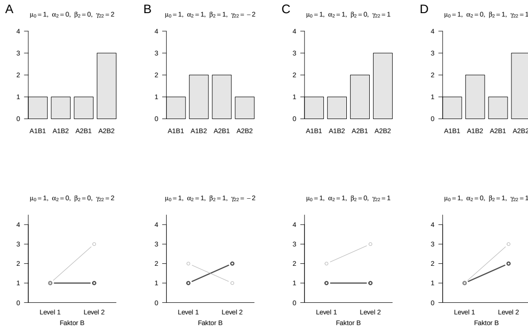
Figure 42.5 Group expectation values of example parameter scenarios in bar- and line-plot form in the two-way ANOVA model with interaction.
