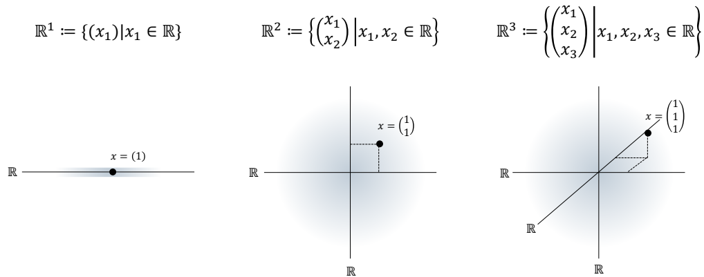
Figure 2.7 \mathbb{R}^n for n = 1 , n = 2 , and n = 3 . The black dots each represent an element of the corresponding set.
