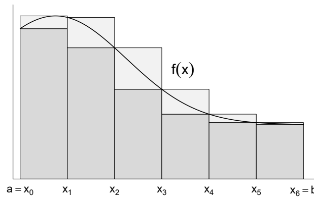
Figure 7.2 Partition and upper and lower Riemann sums
