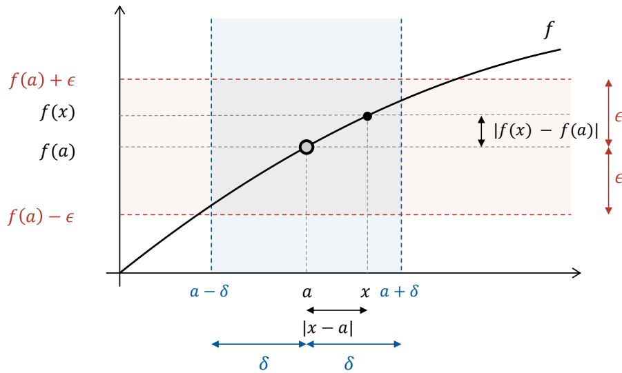
Figure 5.4 For every \epsilon > 0 , a \delta > 0 can be chosen such that, for all x \in D , |x - a| < \delta implies |f(x) - f(a)| < \epsilon .
