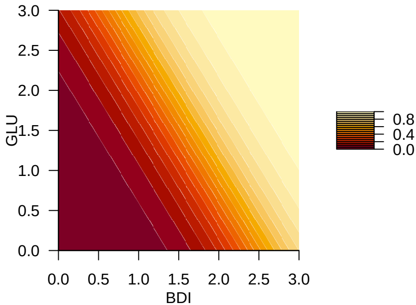
P(Non-Response)
