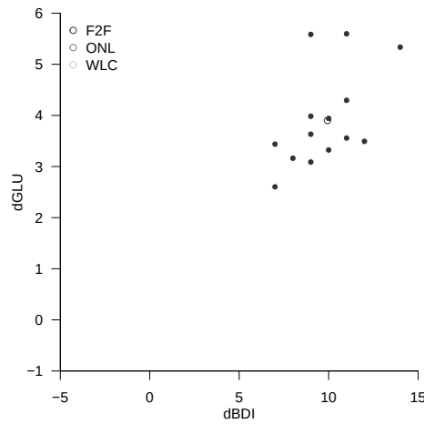
Figure 47.1 Descriptive statistics of the dBDI, dGLU data of the example data set. Each point visualizes the data of one patient. The sample covariance is shown by the 0.7 isocontour of a two-dimensional normal distribution whose expected-value parameter and covariance-matrix parameter correspond to the sample mean and sample covariance of the respective group.
