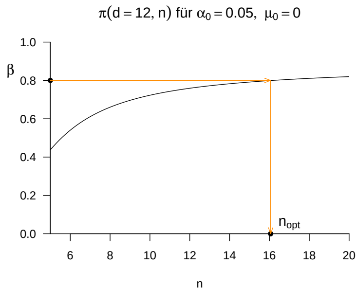
Figure 46.9 Determination of a minimal sample size for detecting a minimum noncentrality-parameter value of \delta_\mu = 12 . The figure shows the corresponding section function of the function shown in Figure 46.8.
