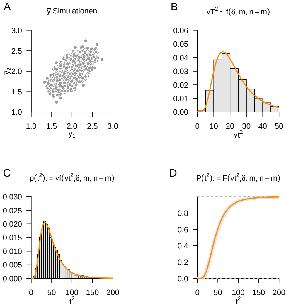
Figure 46.4 Distribution of the one-sample T^2 test statistic. A Sample means of 10,000 realizations of a one-sample T^2 test model with m := 2 and n := 15 and true, but unknown, parameters
