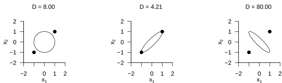
Figure 45.2 Mahalanobis distances as a function of component covariances.
