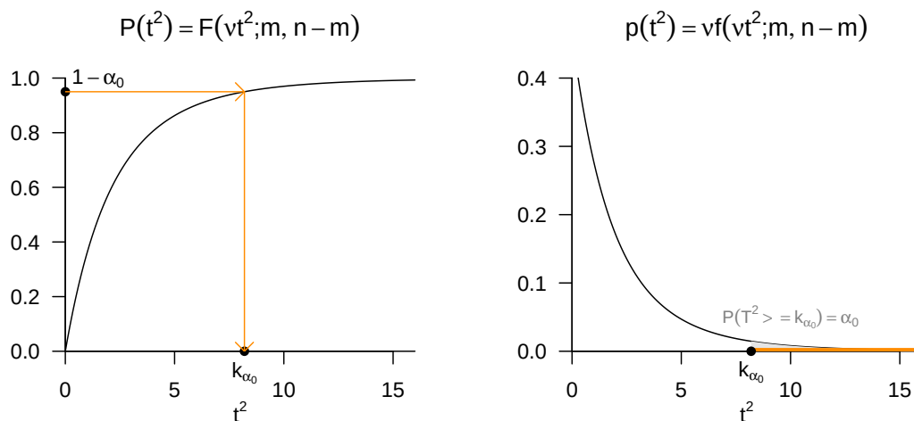
Figure 46.7 Size control by selecting an \alpha_0 -dependent critical value for the one-sample T^2 test using the CDF and PDF of the one-sample T^2 test statistic.
