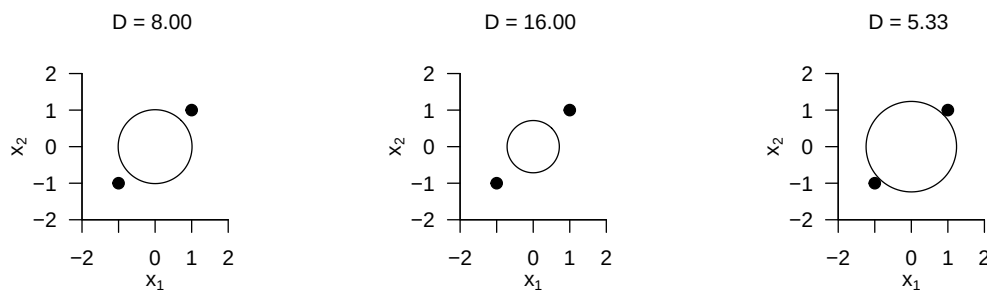
Figure 45.1 Mahalanobis distances as a function of component variances.
