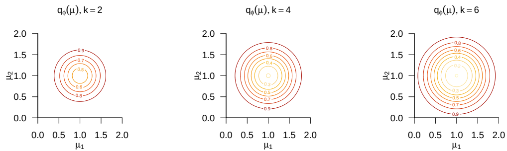
Figure 46.5 One-sample T^2 test power functions for critical values k = 2 , k = 4 , and k = 6 in the scenario
