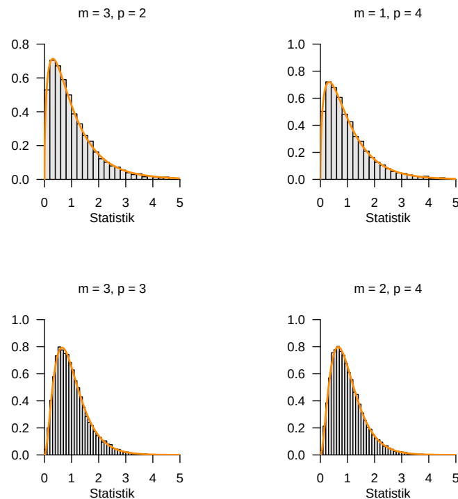
Figure 47.3 Simulation of special distributions of Wilks' \Lambda statistic transformations when the null hypothesis is true.
