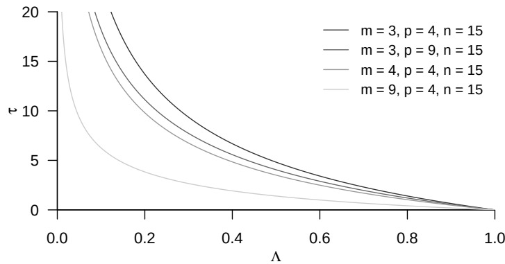
Figure 47.4 Relationship between Wilks' \Lambda statistic and the \tau statistic considered by Rao (1951) in exemplary application scenarios.
