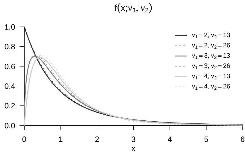
Figure 46.2 Exemplary PDFs of an f random variable.
