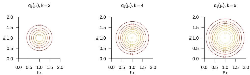
Figure 46.6 One-sample T^2 test power functions for critical values k = 2 , k = 4 , and k = 6 in the scenario
