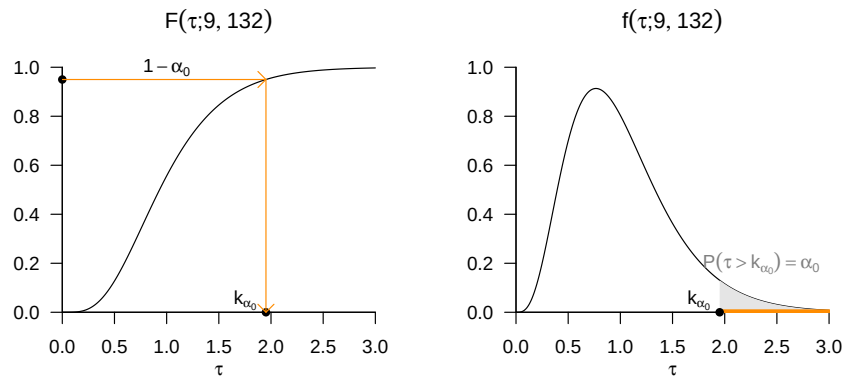
Figure 47.6 Size control by selecting an \alpha_0 -dependent critical value for the Wilks' \Lambda statistic-based test using the CDF and PDF of the transformed Wilks' \Lambda statistic \tau .
