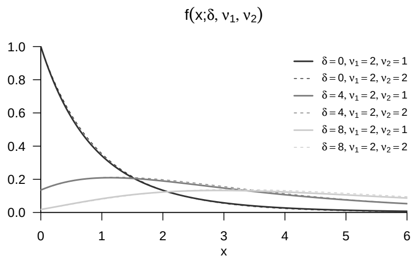
Figure 46.3 Exemplary PDFs of a noncentral f random variable.
