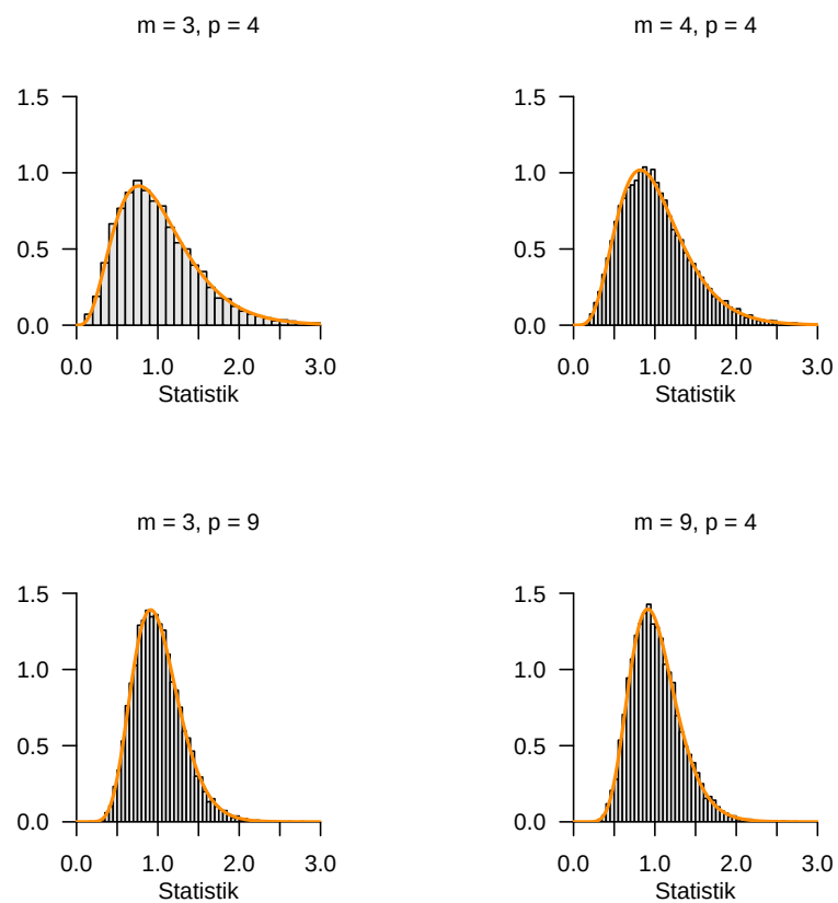
Figure 47.5 Simulation of approximate distributions of Wilks' \Lambda statistic transformations when the null hypothesis is true.
