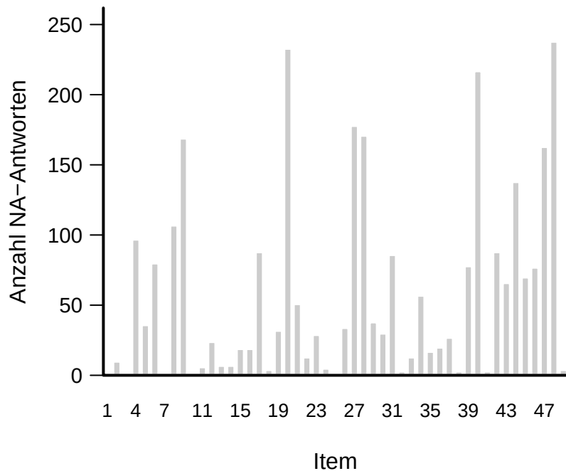
Dichotome Items (m = 49, NA-Mittel = 58.4)
