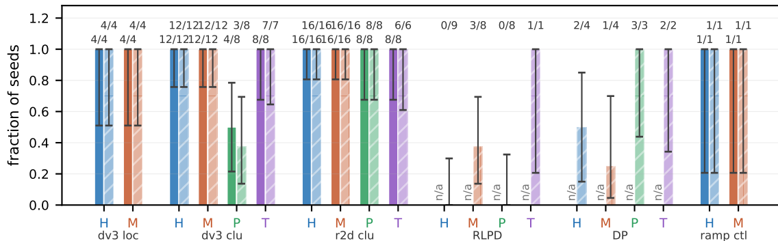
Ignition rate by condition, observation pixels, ladder nested_sparse10
