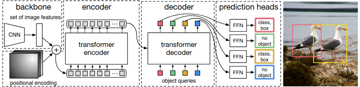
Figure 2.1: DETR architecture [3].
