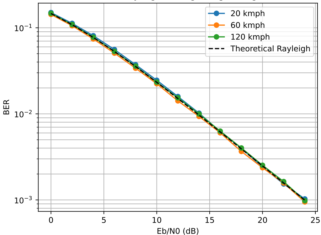
BER vs SNR under Rayleigh Fading using Zheng-Xiao's Model
