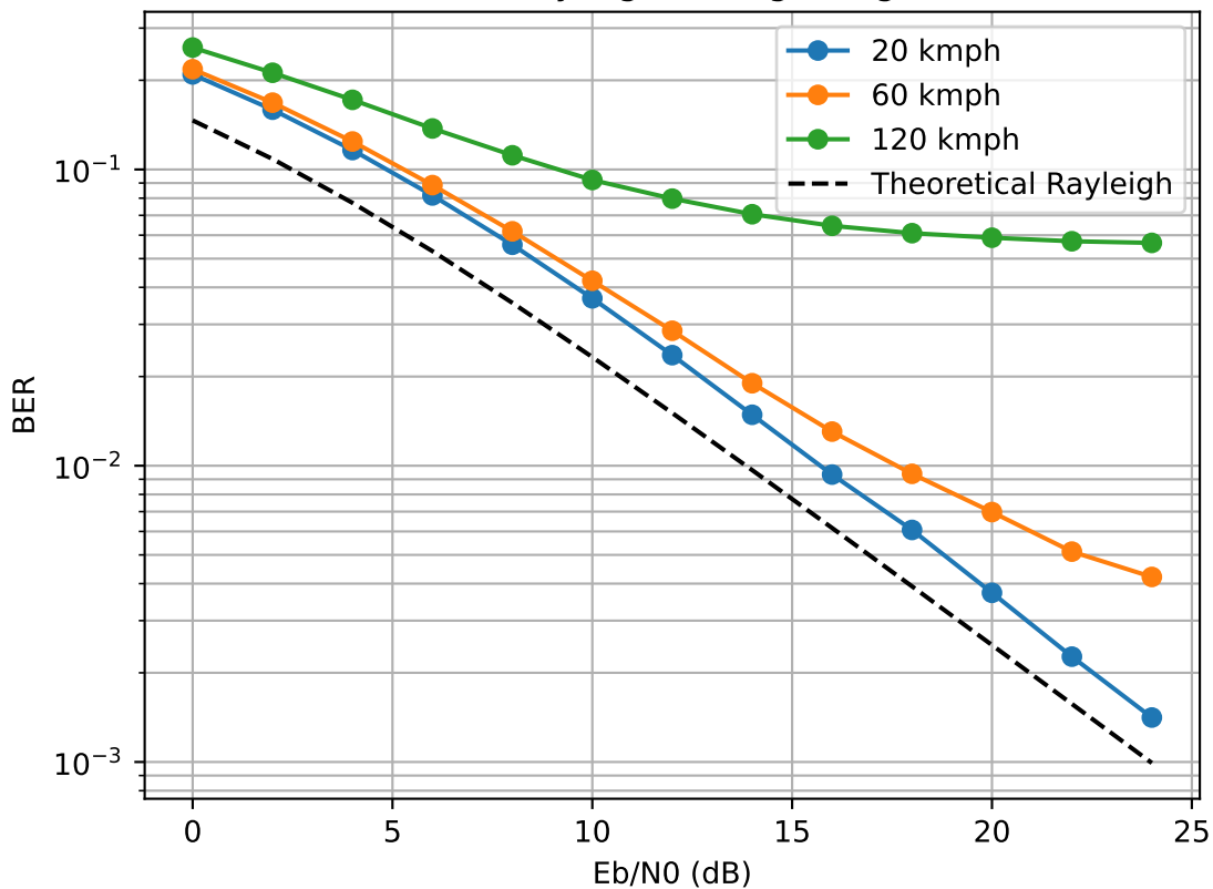
BER vs SNR under Rayleigh Fading using Smith's Model
