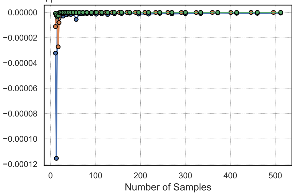
R 2
