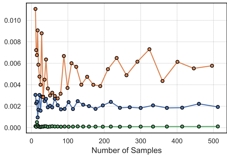
R 2
