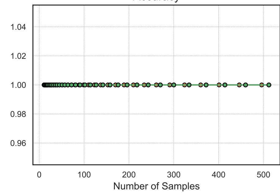
Accuracy
