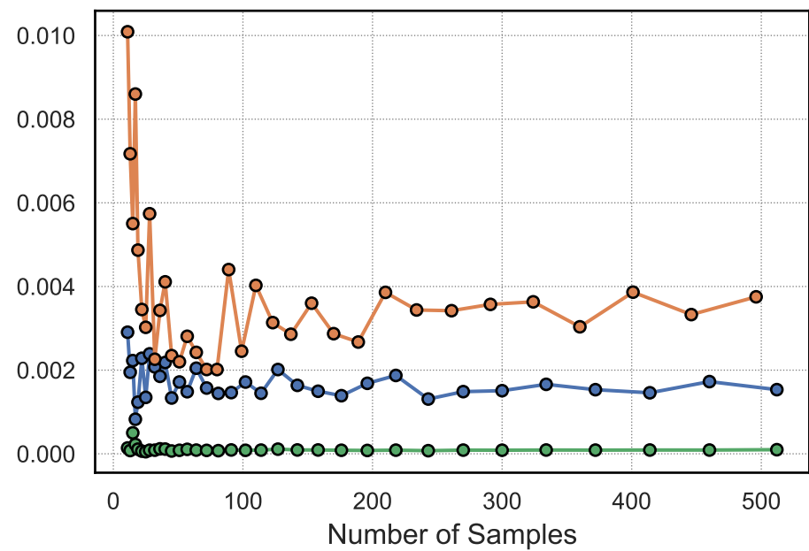
Accuracy
