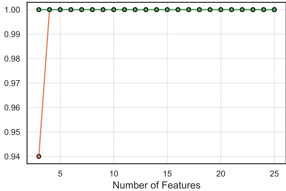
Accuracy
