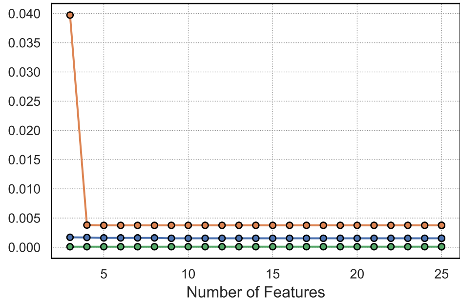
Accuracy
