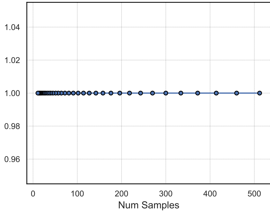
Accuracy
