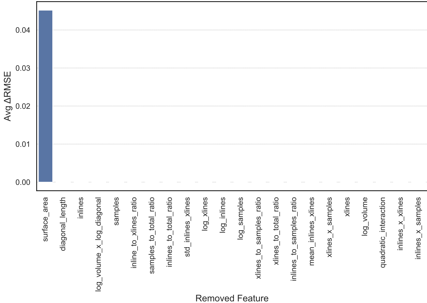
Impact of Removing Each Feature on RMSE - gst3d
