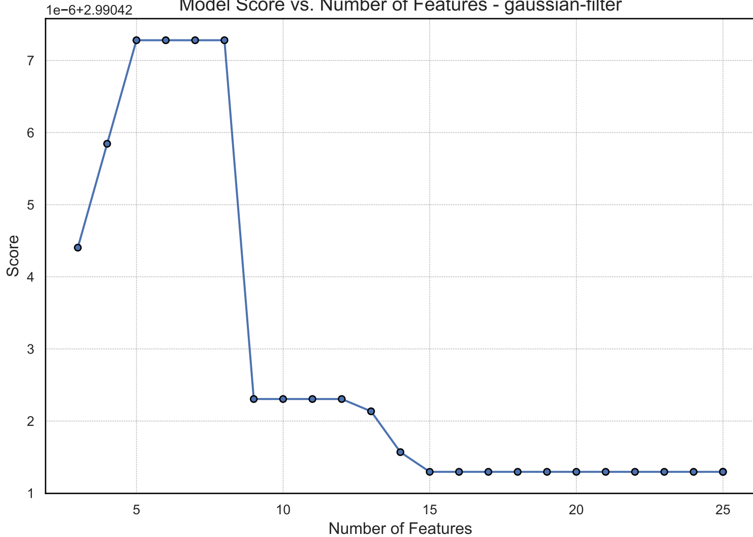
Model Score vs. Number of Features - gaussian-filter
