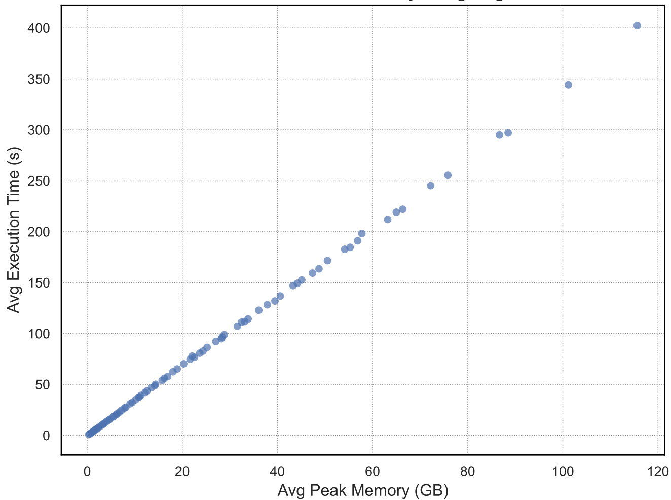
Execution Time vs. Memory Usage - gst3d
