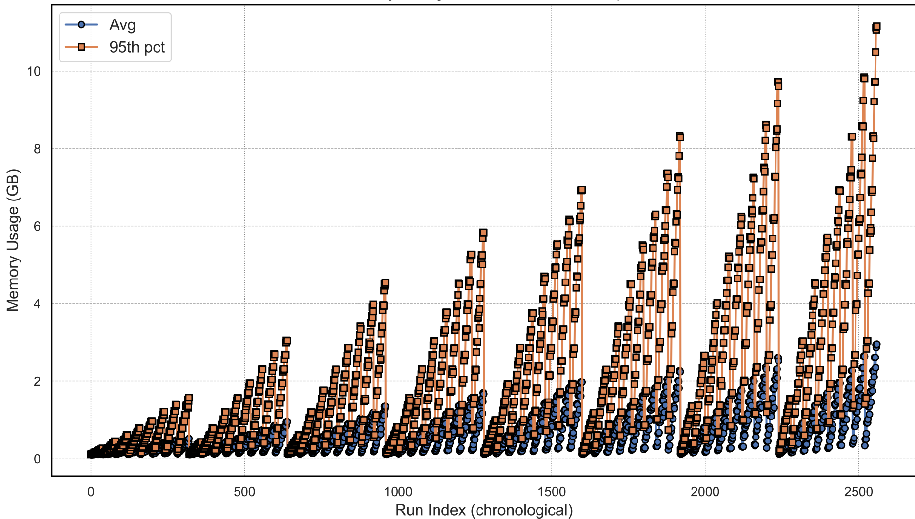
Memory Usage Over Runs - envelope
