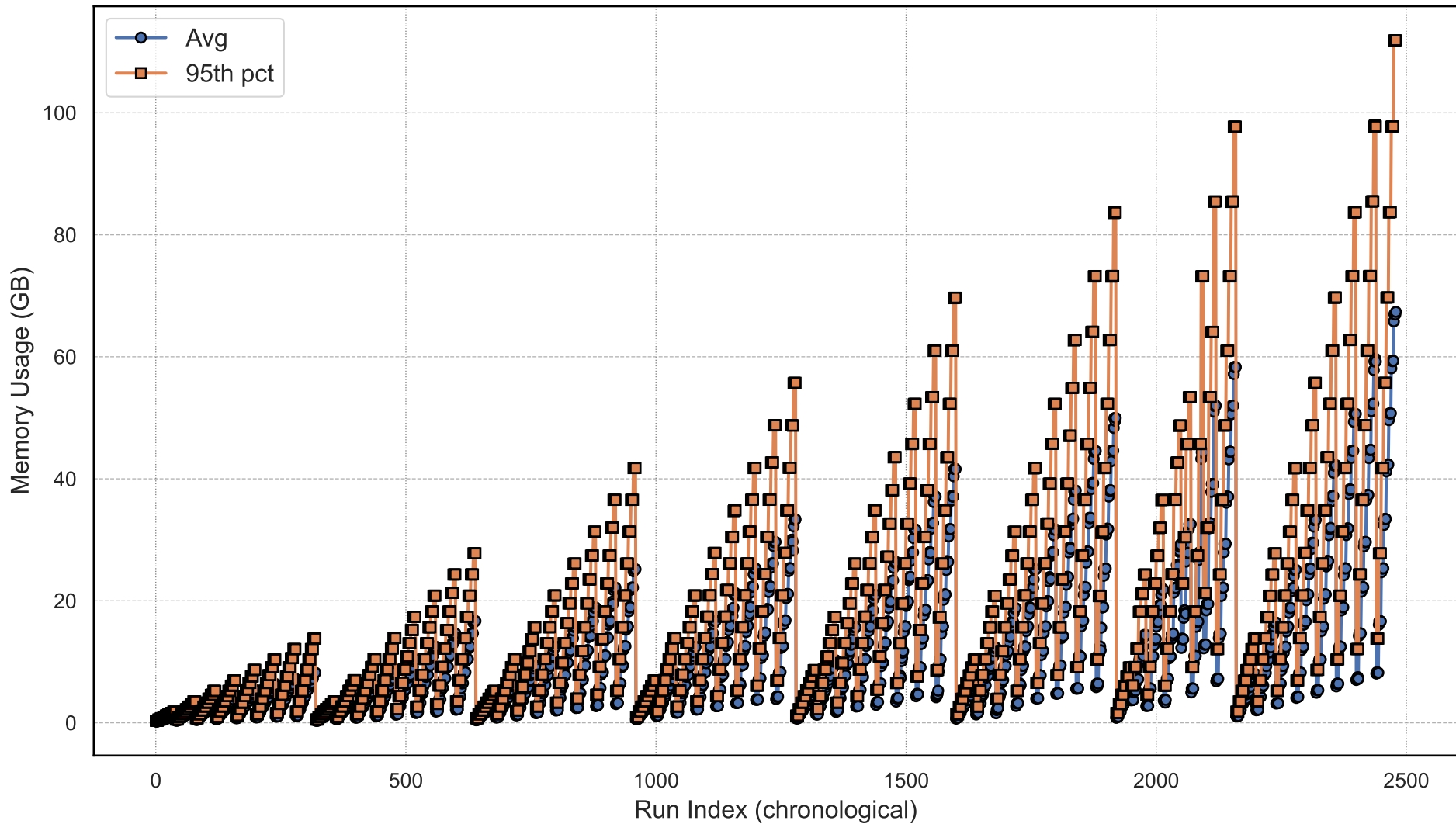
Memory Usage Over Runs - gst3d
