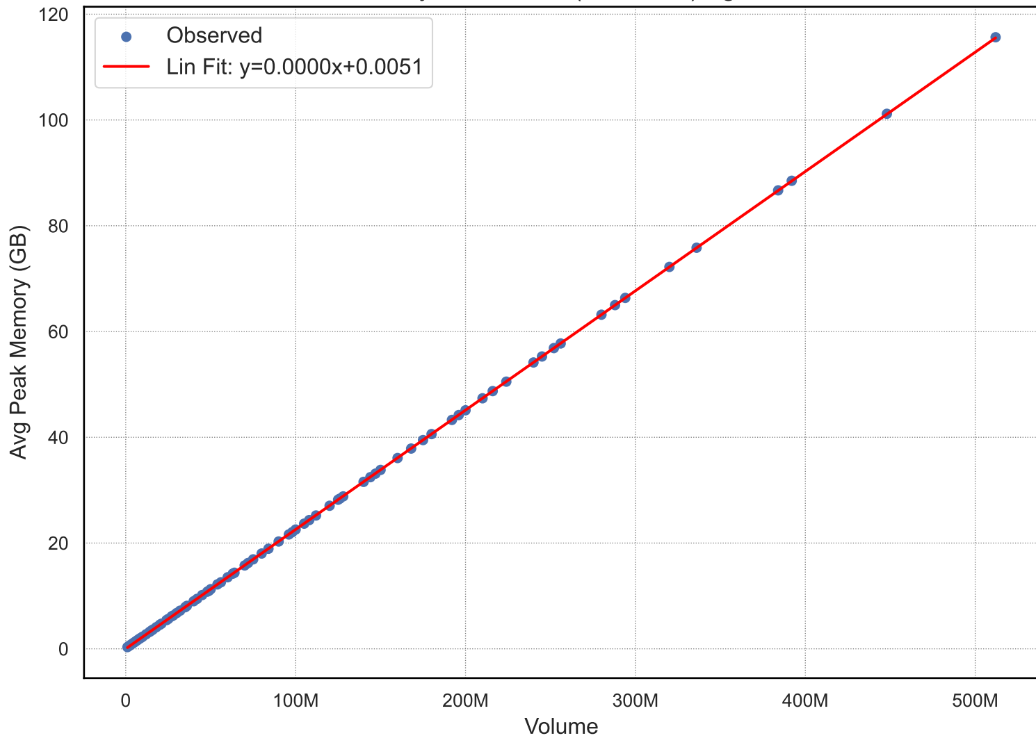
Memory vs. Volume (Linear Fit) - gst3d
