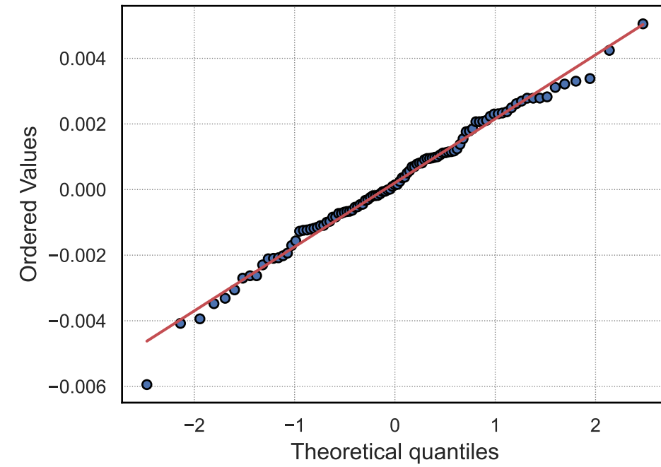
QQ-Plot: random_forest
