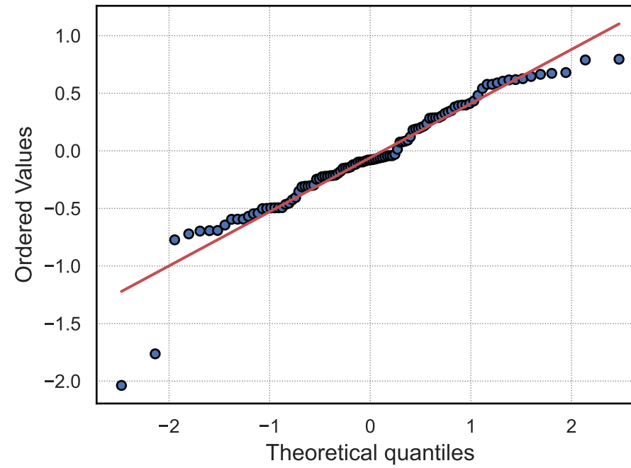
QQ-Plot: gradient_boosting
