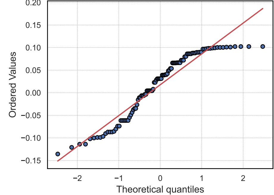
QQ-Plot: support_vector_regression
