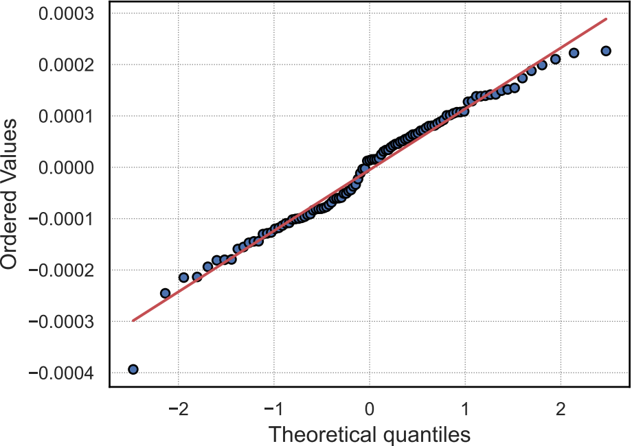
QQ-Plot: random_forest
