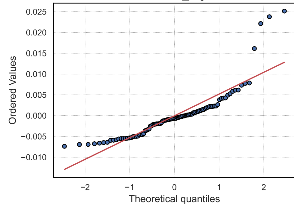
QQ-Plot: random_forest
