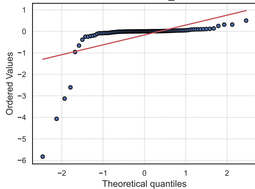
QQ-Plot: support_vector_regression
