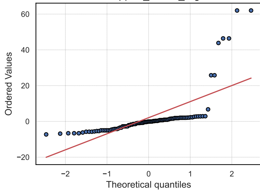
QQ-Plot: support_vector_regression
