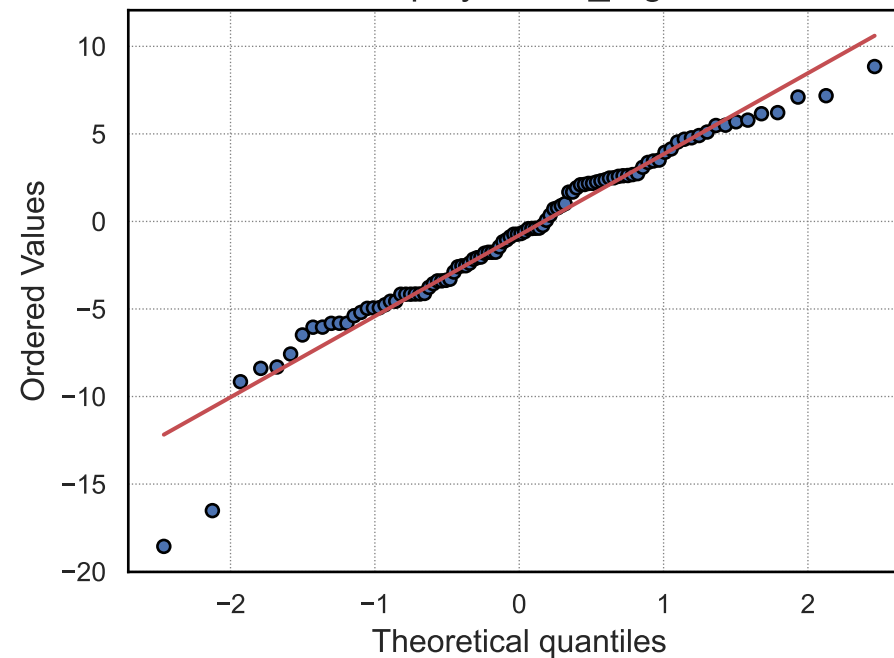
QQ-Plot: gradient_boosting
