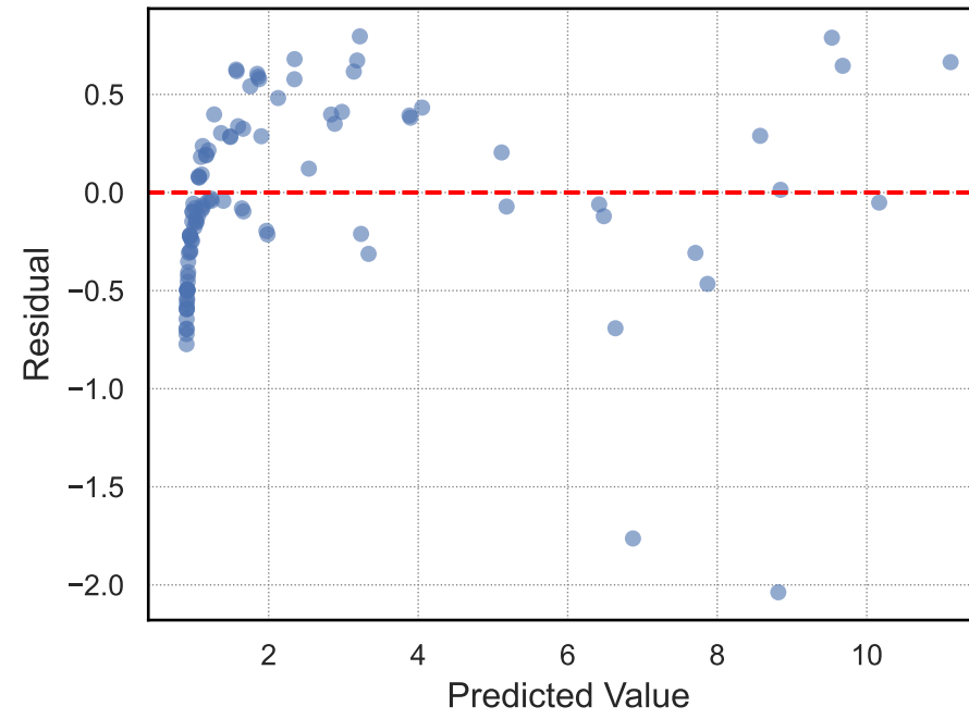
gradient_boosting
