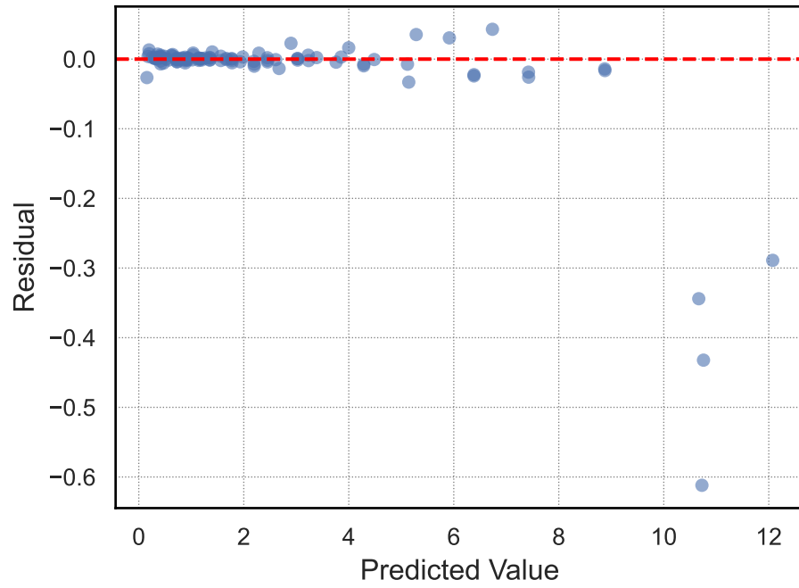
support_vector_regression
