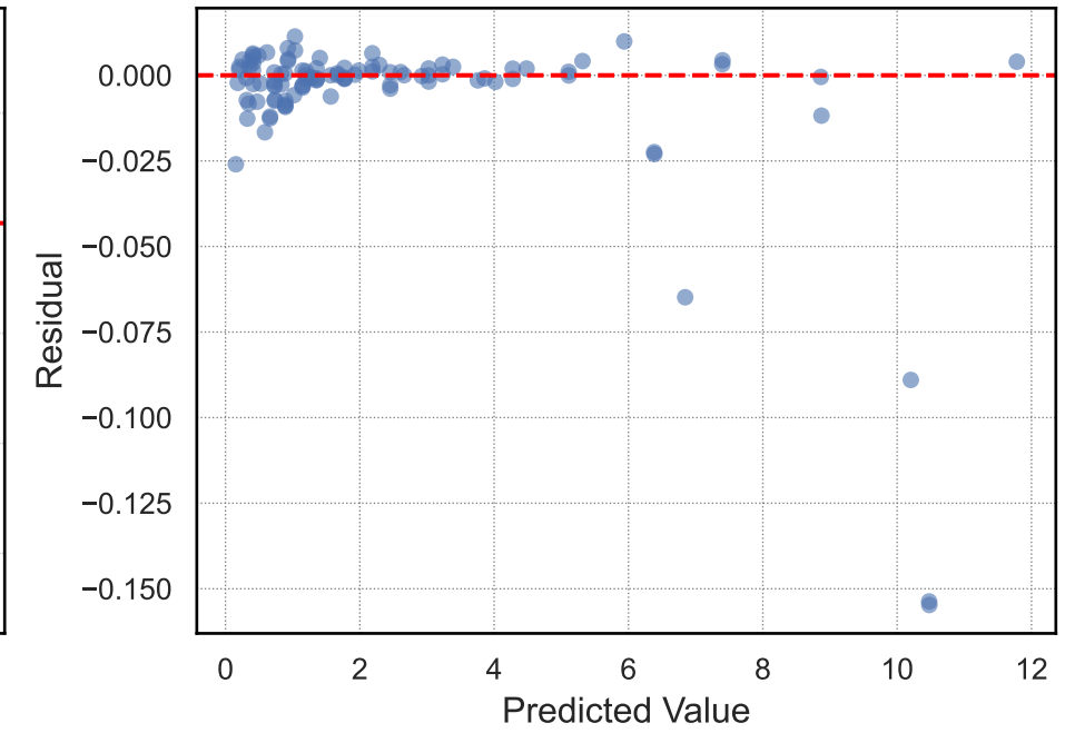
xgboost
