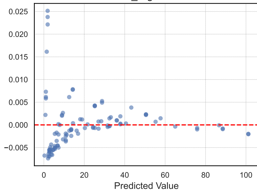
random_forest
