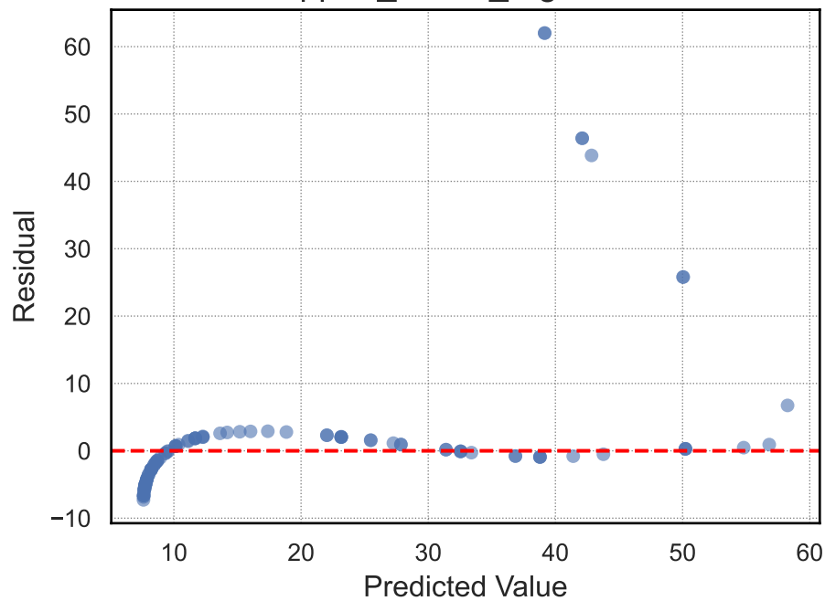
support_vector_regression
