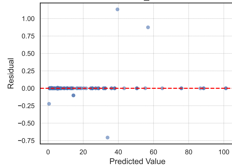
xgboost
