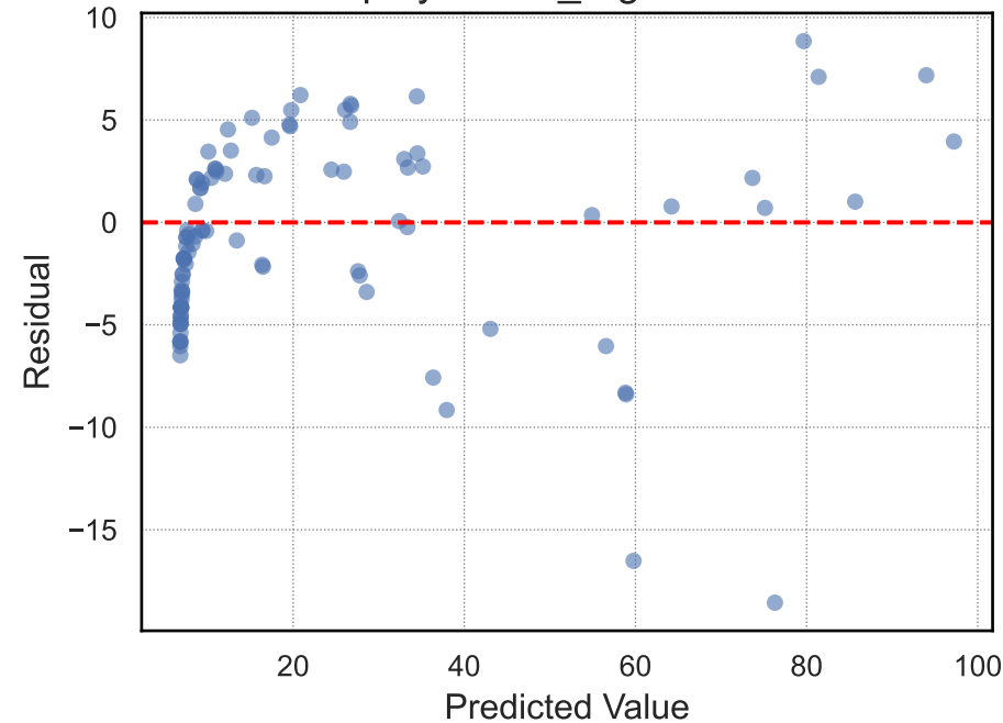
gradient_boosting
