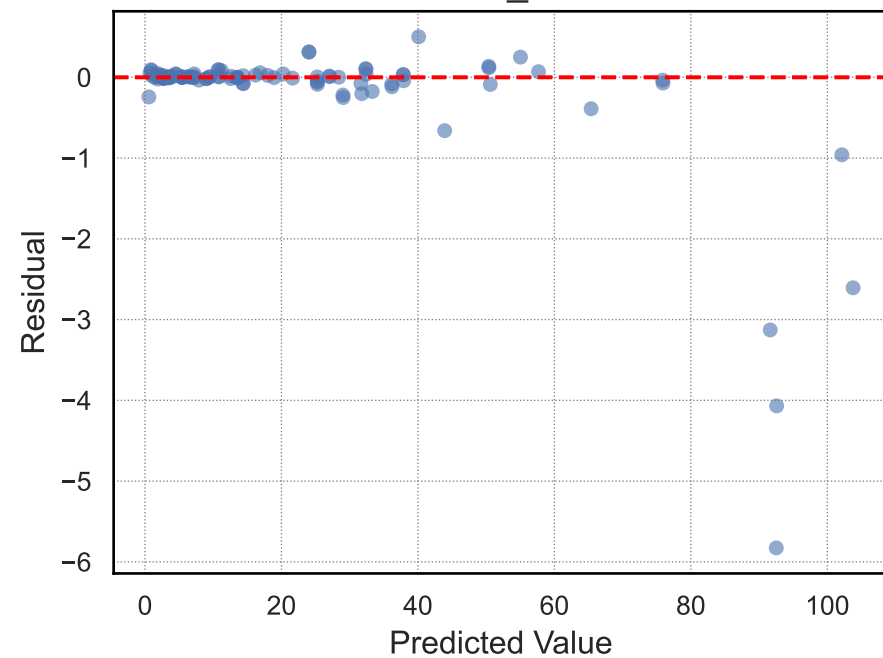
support_vector_regression
