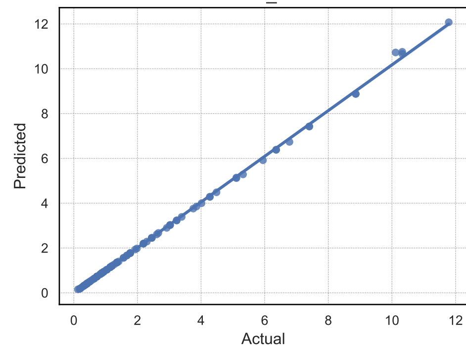
support_vector_regression
