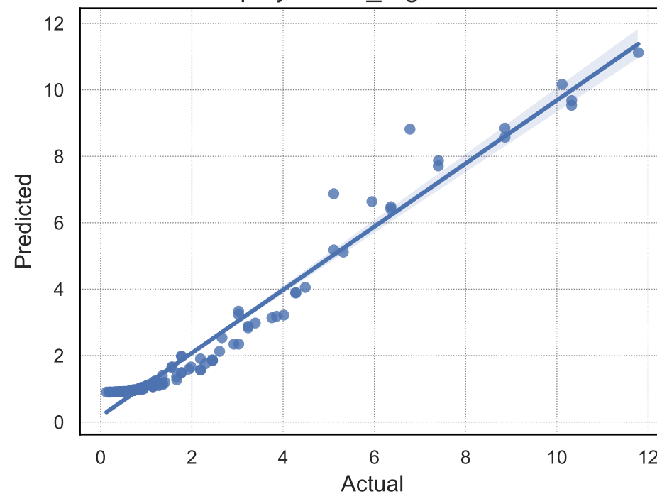
gradient_boosting
