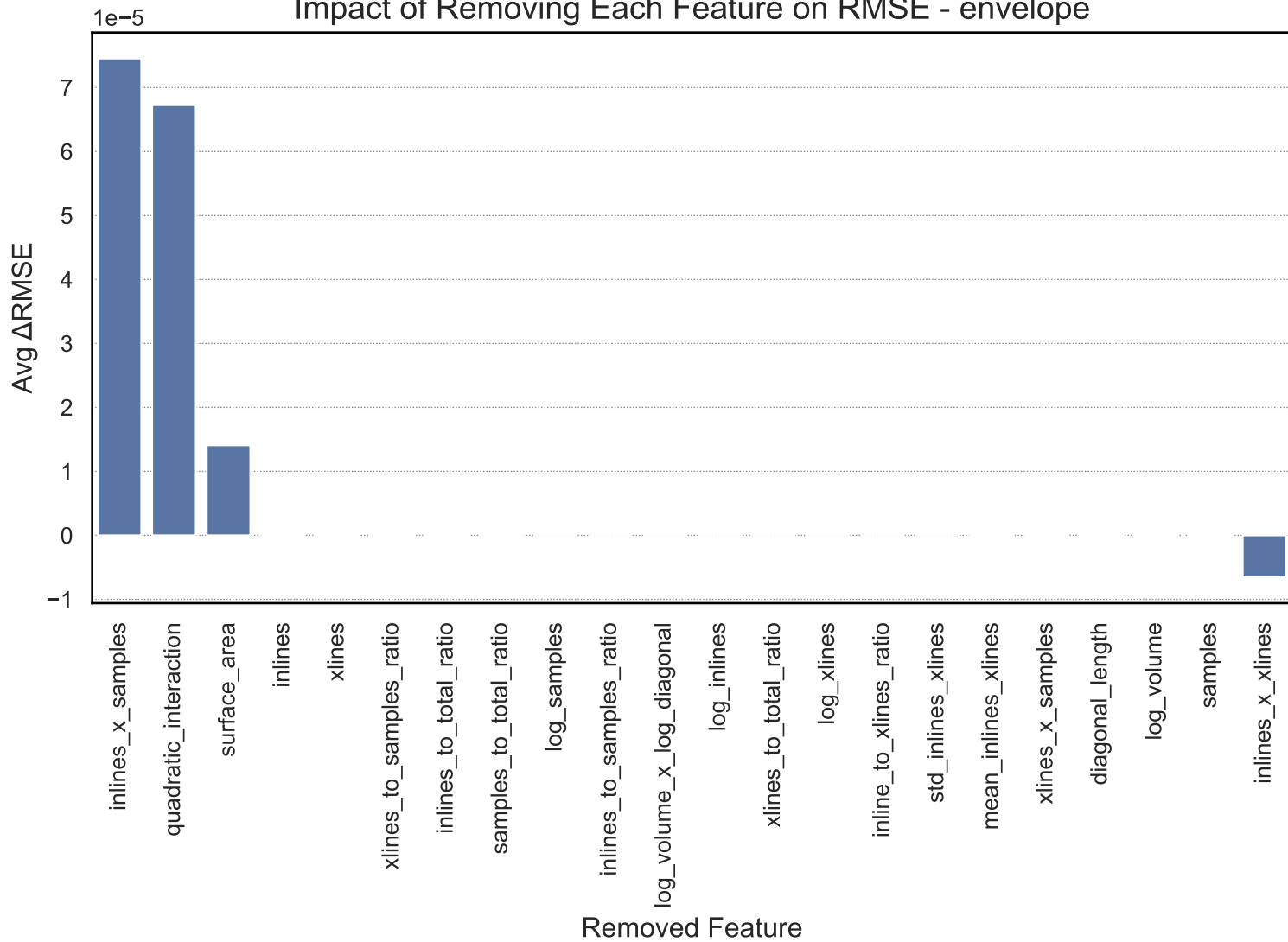
Impact of Removing Each Feature on RMSE - envelope
