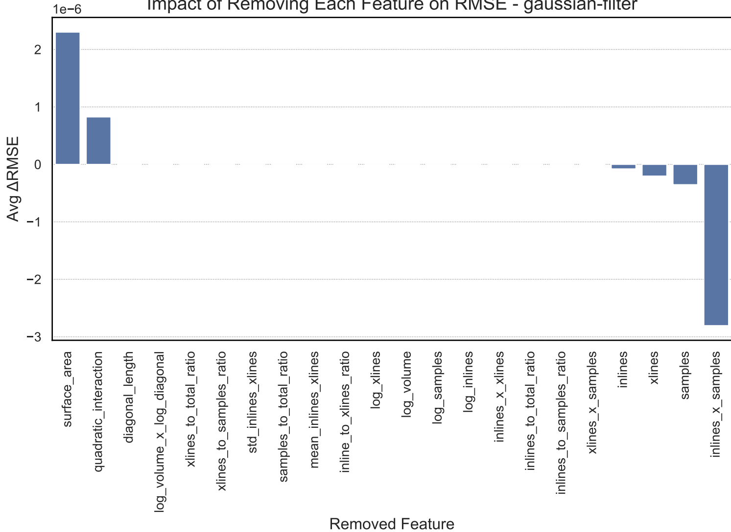
Impact of Removing Each Feature on RMSE - gaussian-filter
