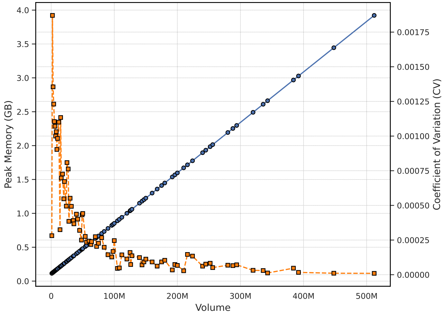
Peak Memory Usage (GB) - gaussian-filter
