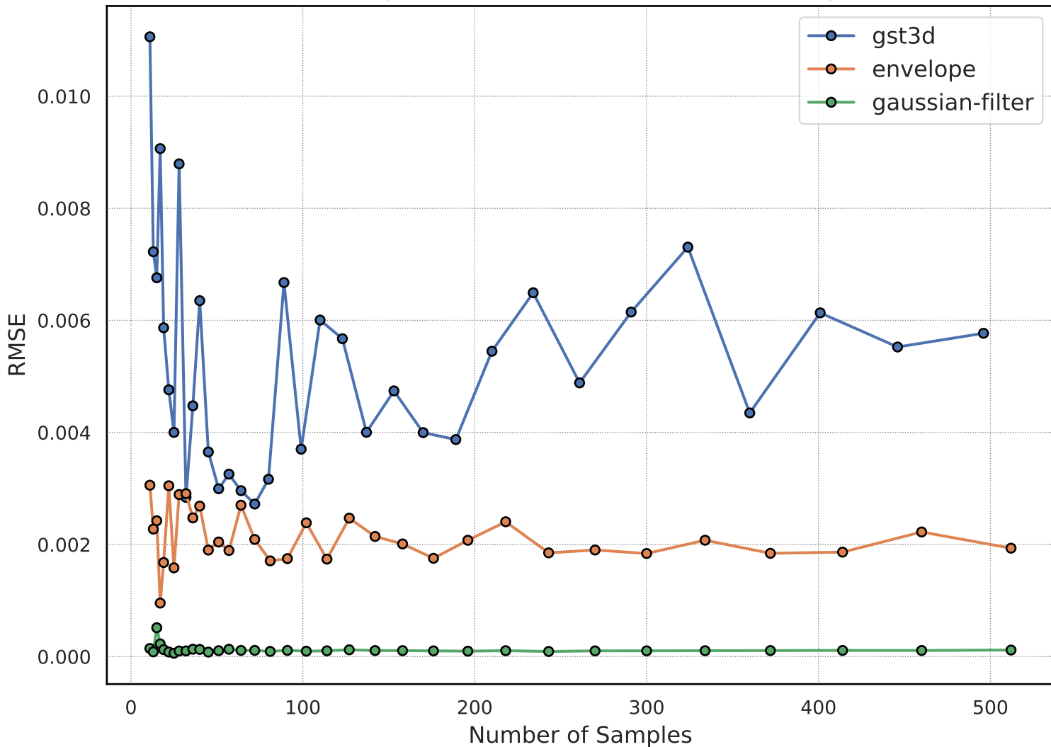
Cross-Operator: RMSE vs Number of Samples
