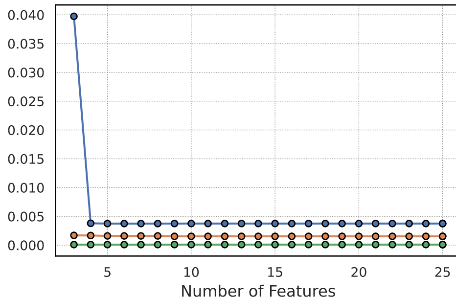
Accuracy
