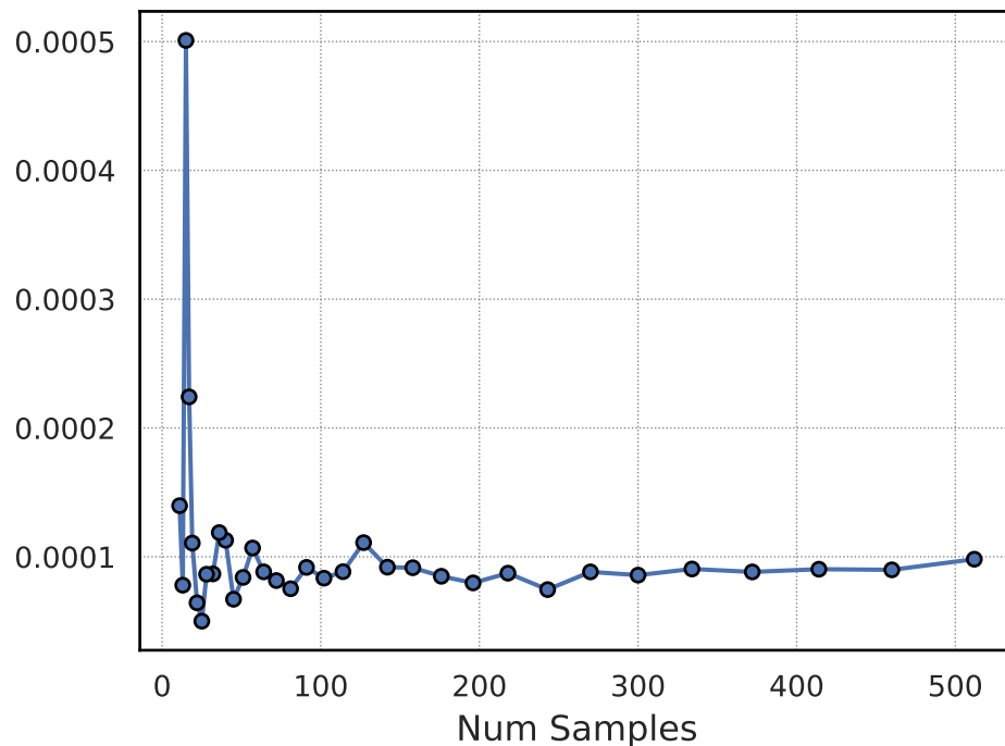
Accuracy
