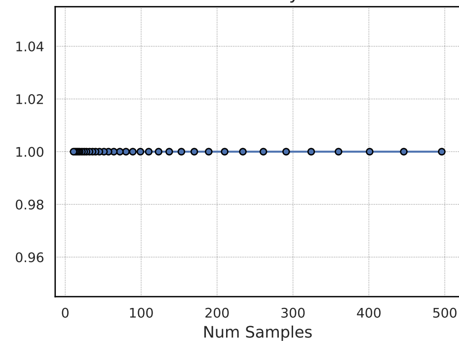
Accuracy
