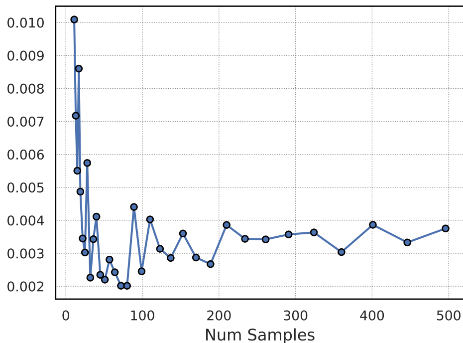
Accuracy
