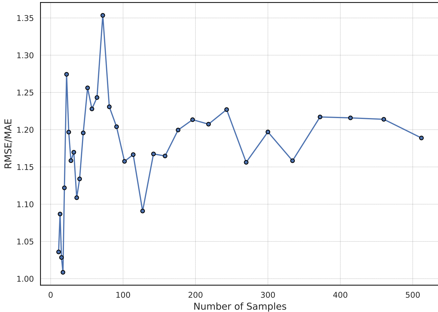
RMSE/MAE Ratio Over Data Reduction - gaussian-filter
