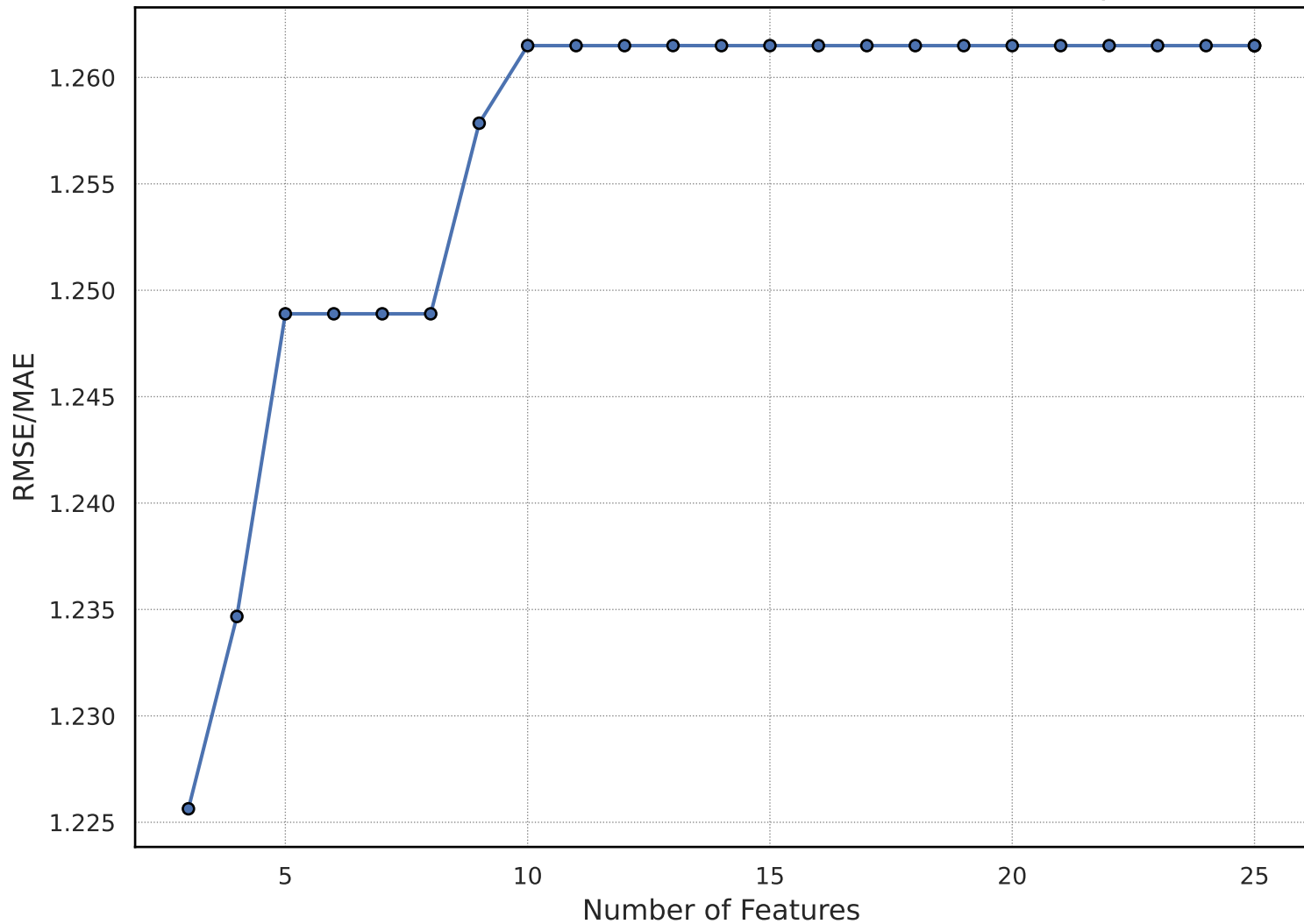
RMSE/MAE Ratio Over Feature Selection - envelope
