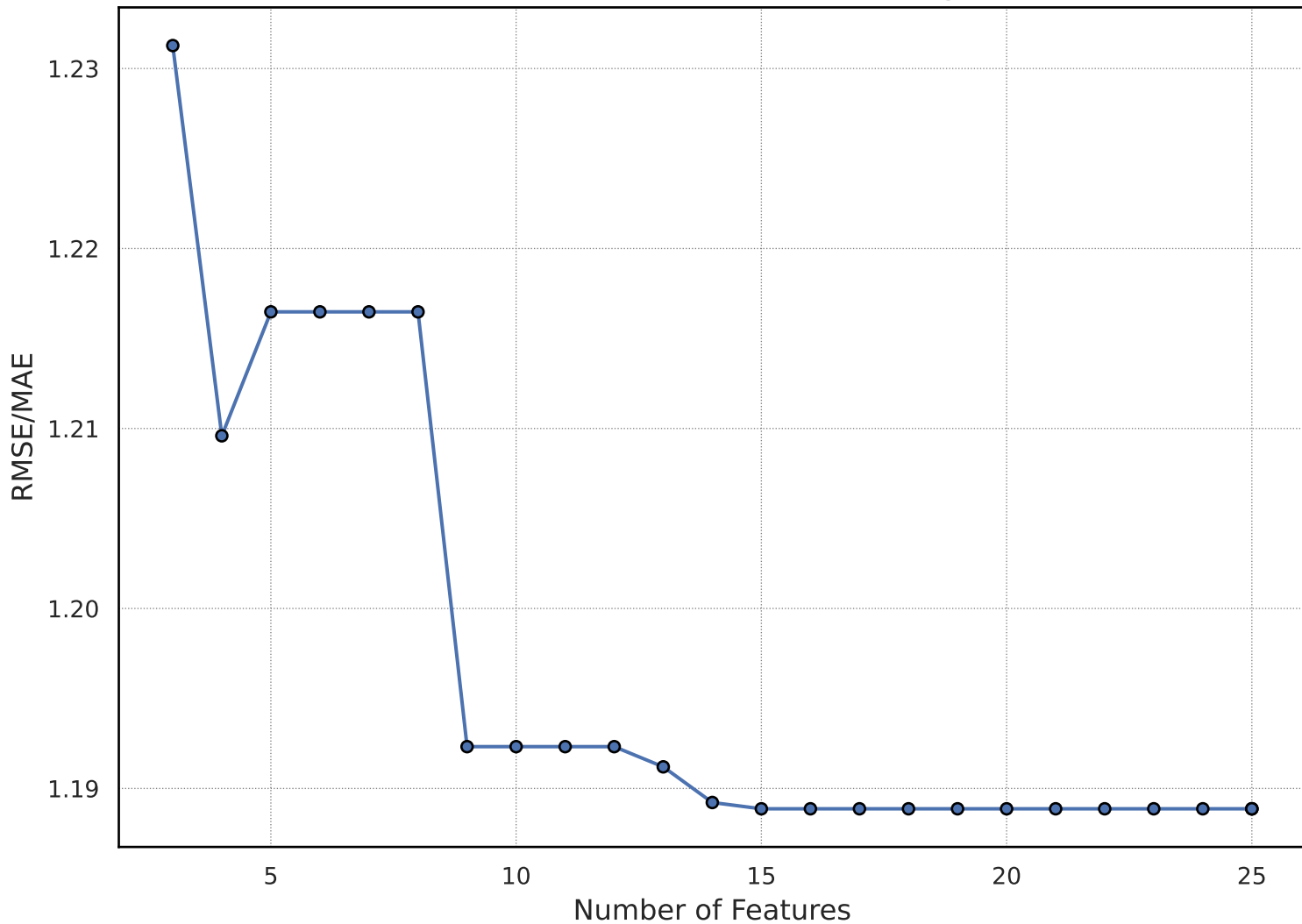
RMSE/MAE Ratio Over Feature Selection - gaussian-filter
