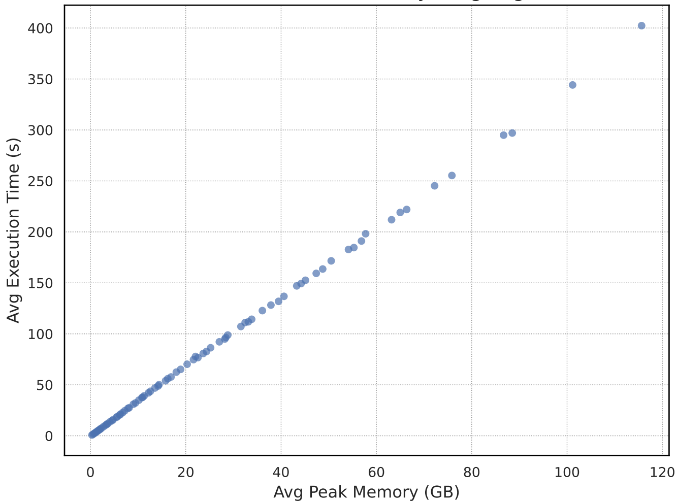
Execution Time vs. Memory Usage - gst3d
