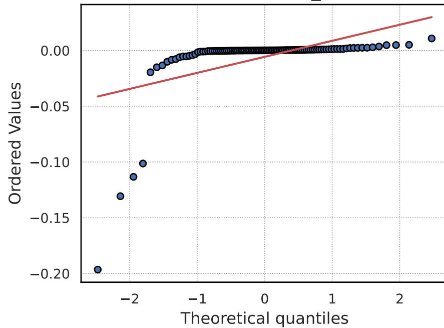
QQ-Plot: support_vector_regression
