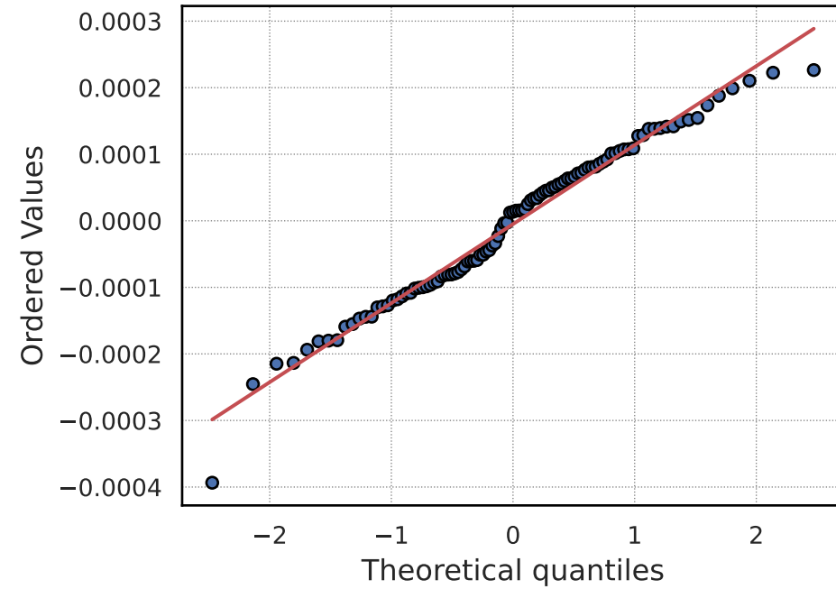
QQ-Plot: random_forest
