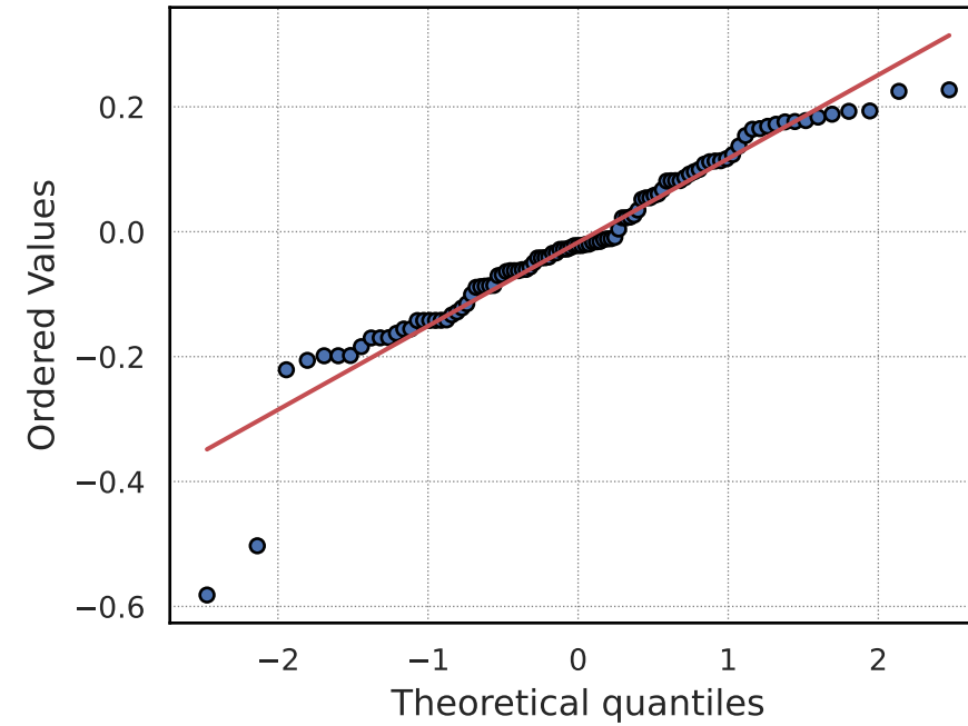
QQ-Plot: gradient_boosting
