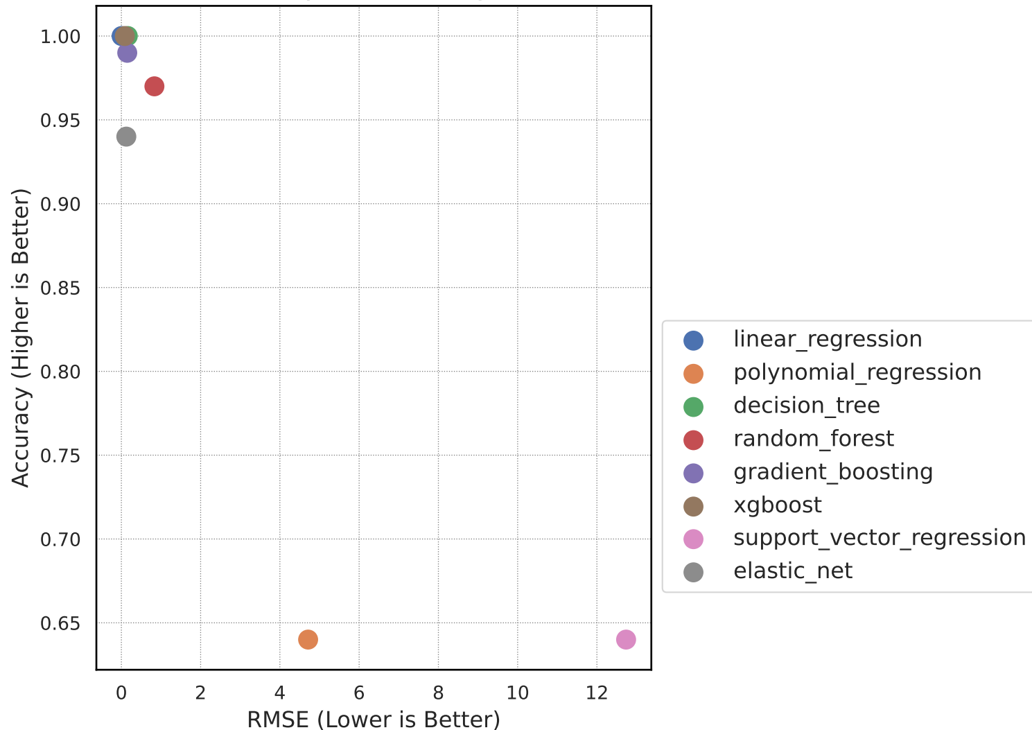
Accuracy vs. RMSE - gst3d
