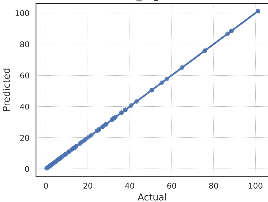
random_forest
