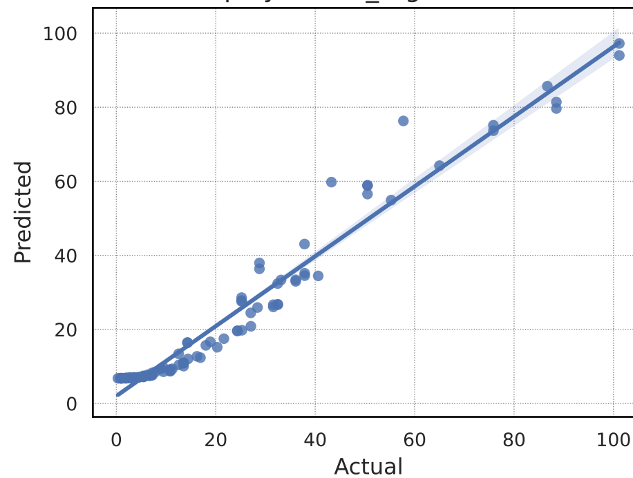
gradient_boosting
