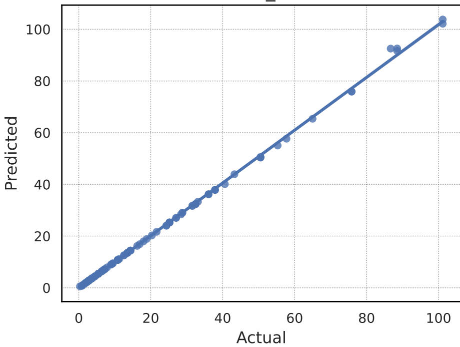
support_vector_regression
