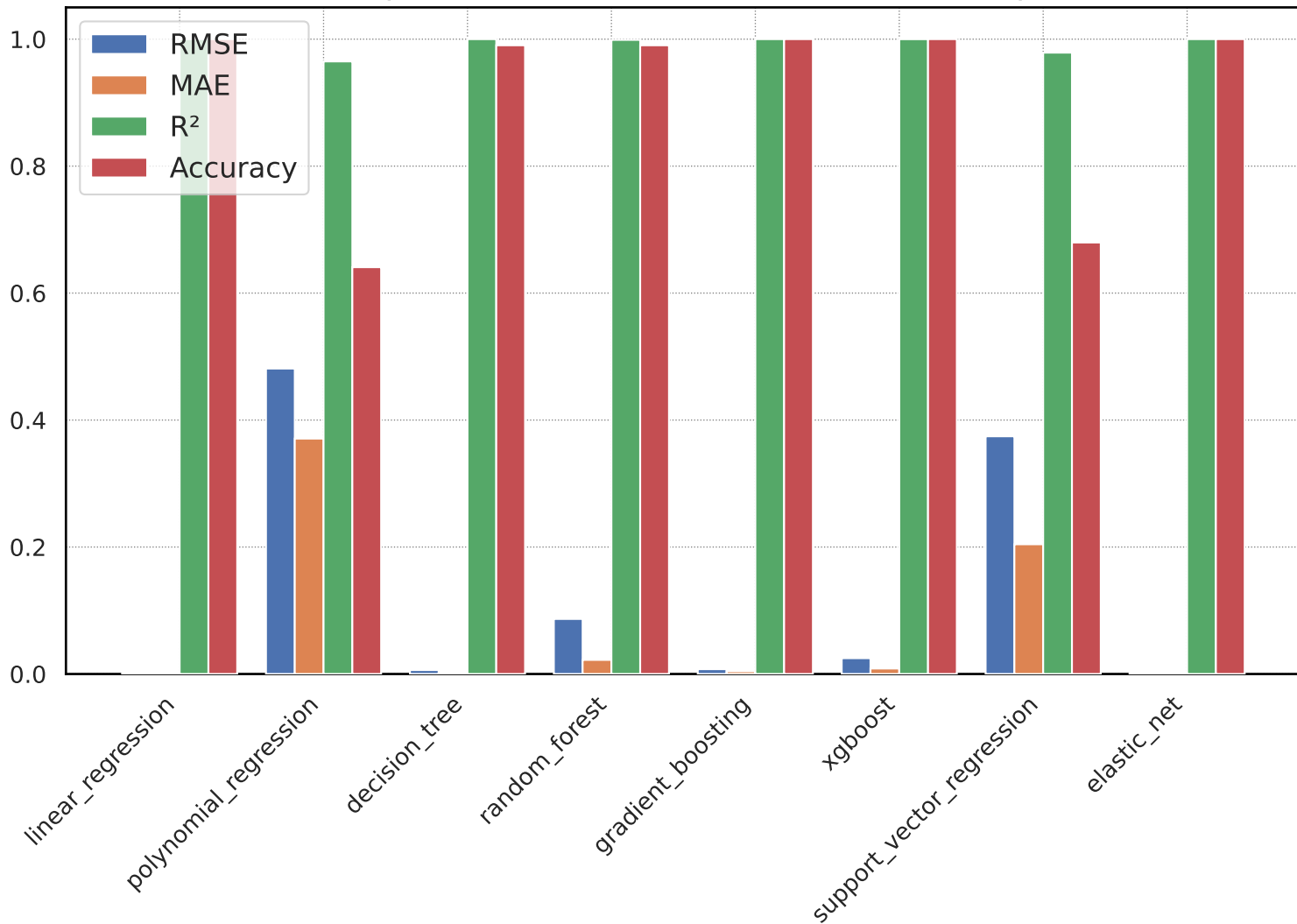
Comparison of Model Performance - envelope
