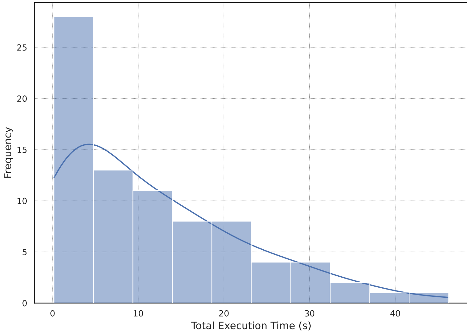
Execution Time Distribution - gaussian-filter
