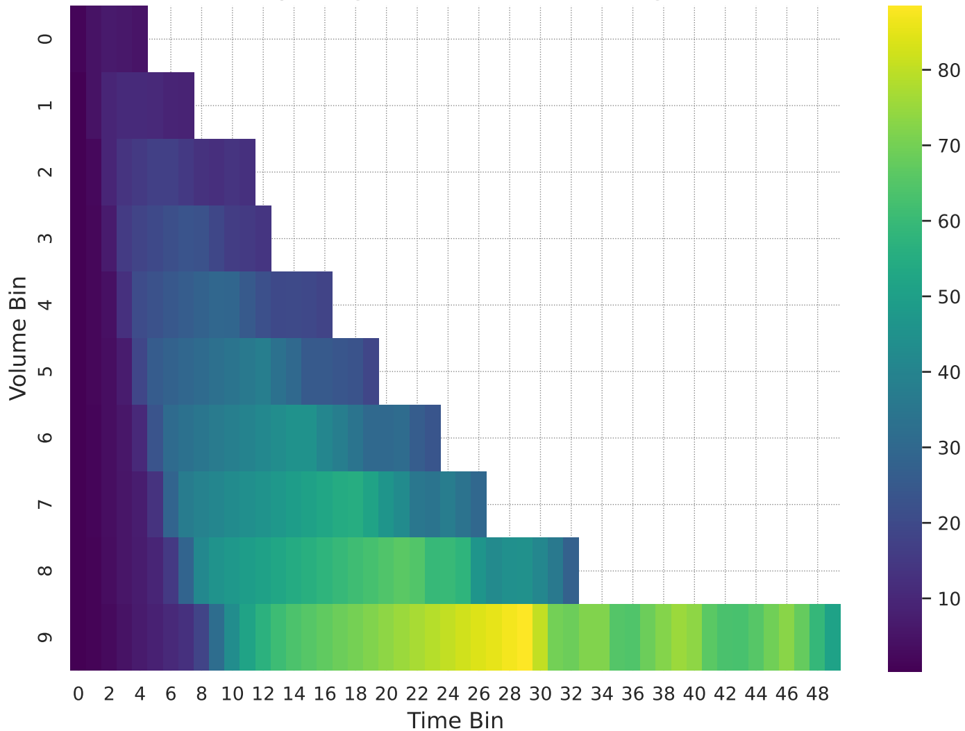
Memory Usage Over Time (Mean) - gst3d
