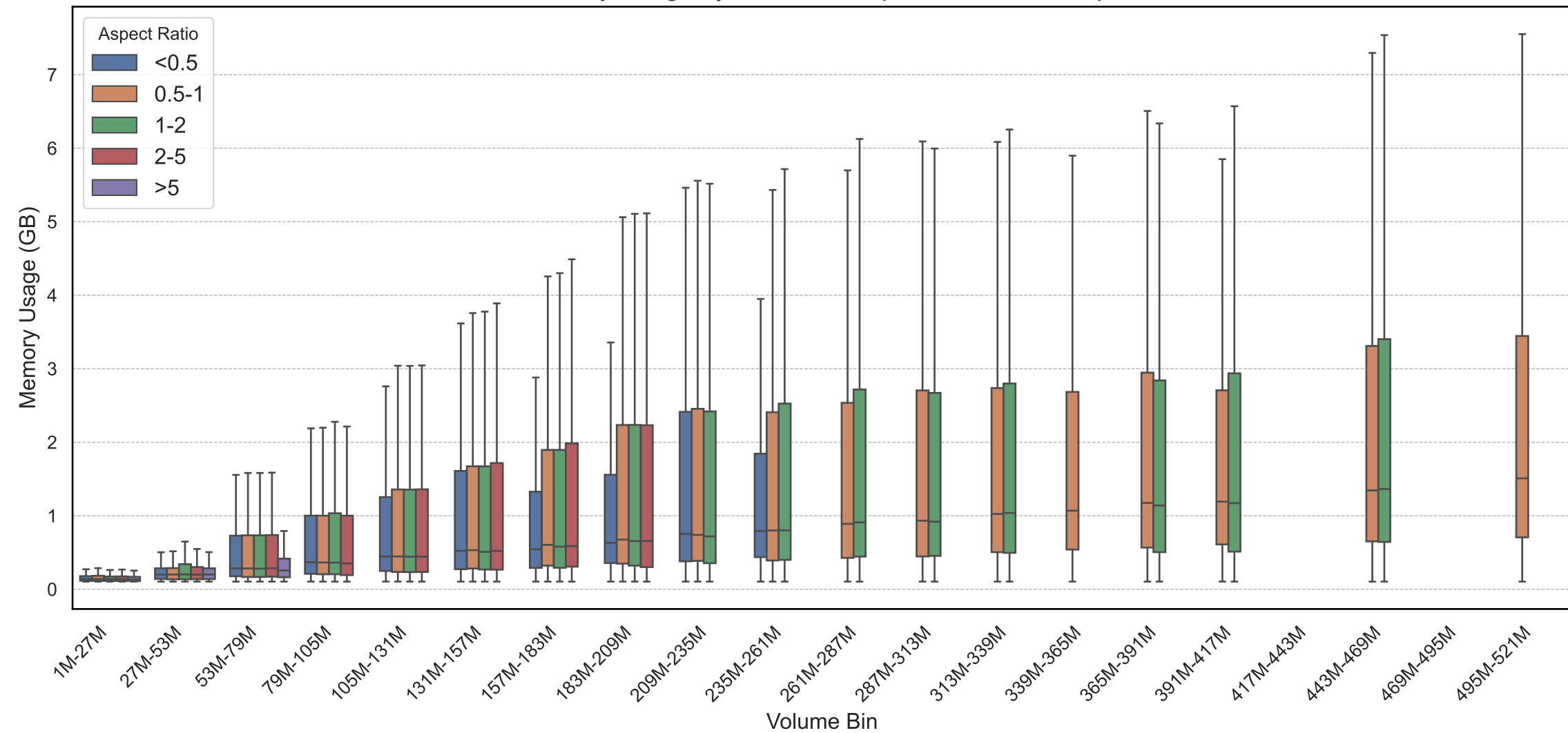
Memory Usage by Volume &amp; Aspect Ratio - envelope
