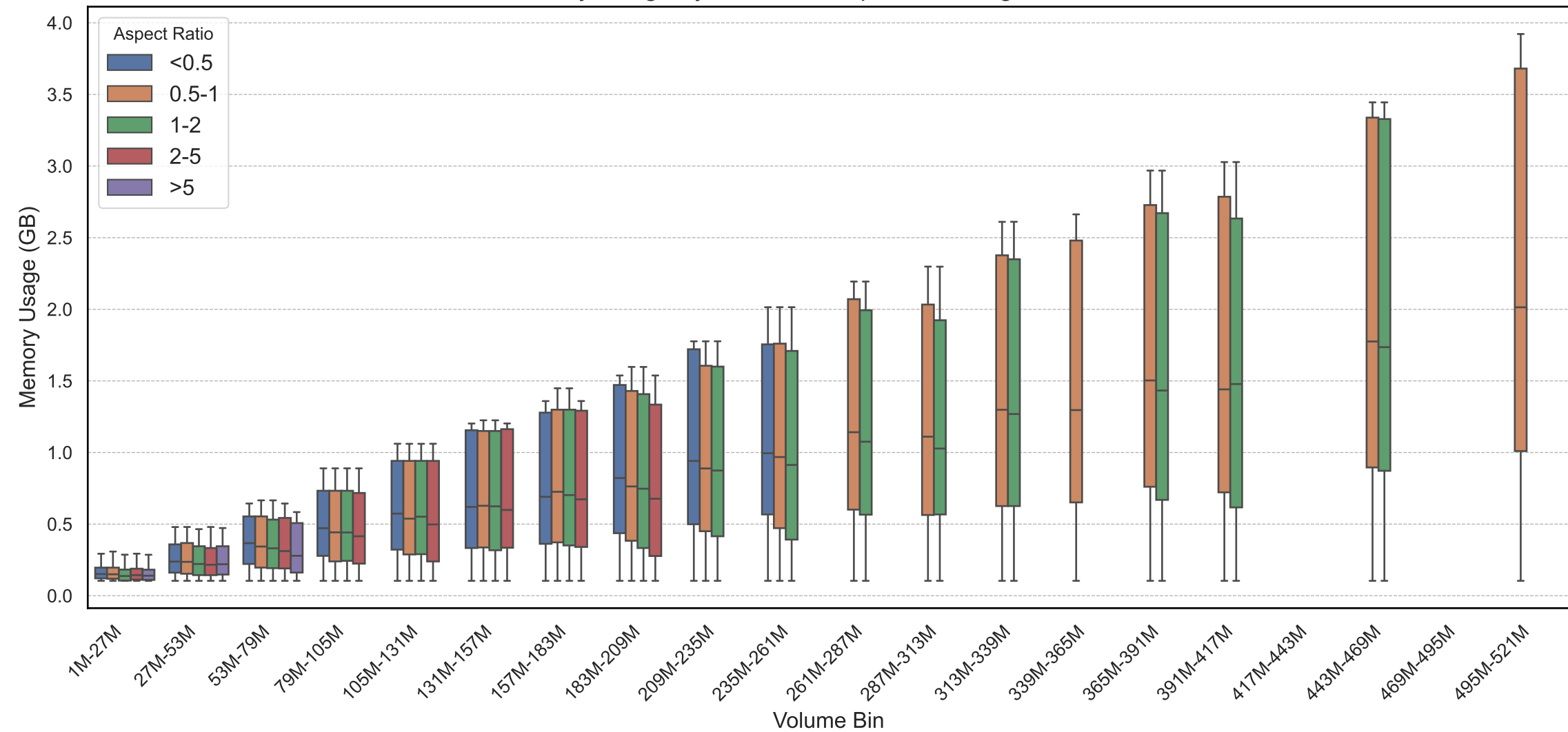
Memory Usage by Volume &amp; Aspect Ratio - gaussian-filter
