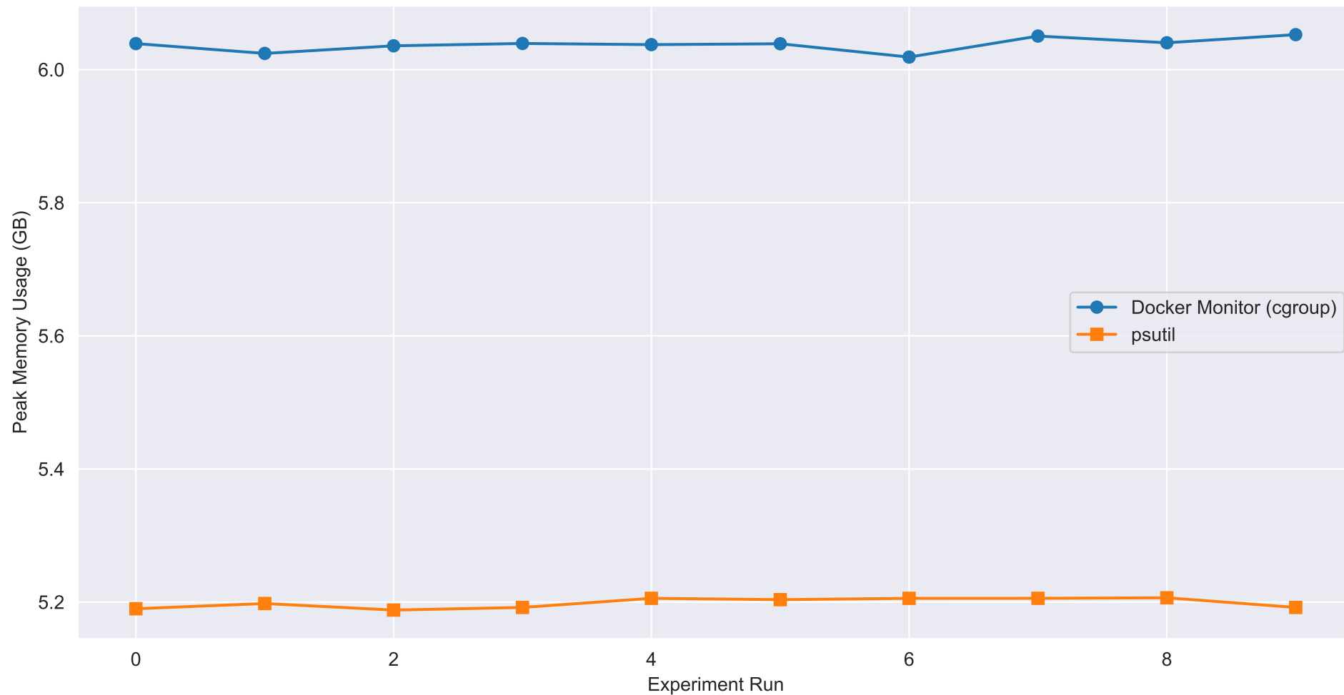
Comparison of psutil vs. Docker cgroup Memory Profiling
