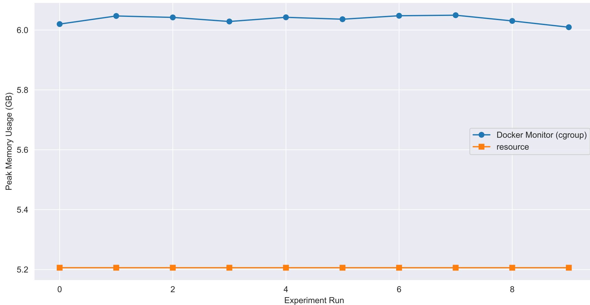
Comparison of resource vs. Docker cgroup Memory Profiling
