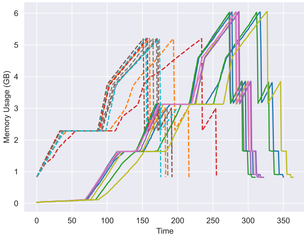
Memory Usage Over Time (psutil vs. Docker cgroup)
