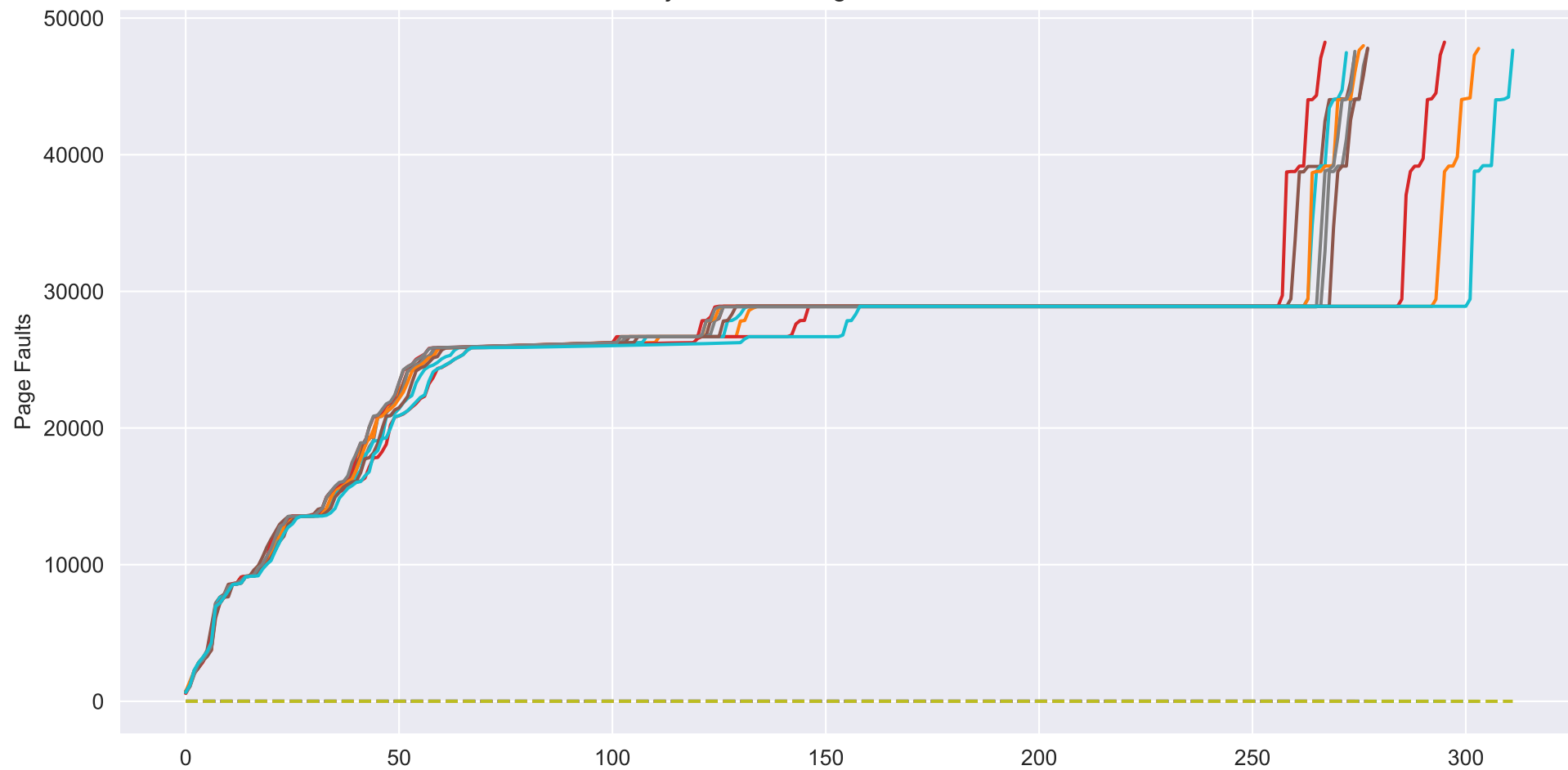
Major & Minor Page Faults Over Time
